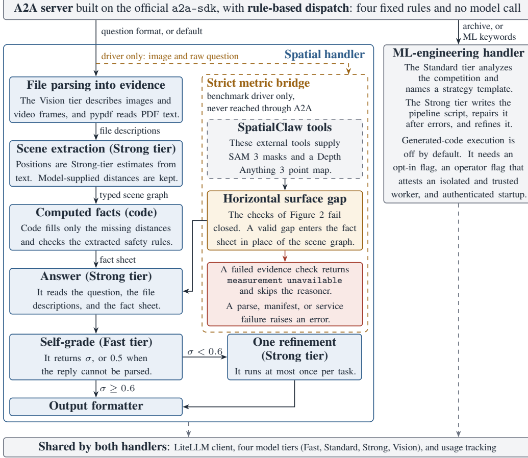
Figure 1: Spatial Atlas places two handlers behind one A2A server. The server passes each task to one handler through four fixed dispatch rules, and no model call takes part in dispatch. On the default spatial path, the Strong tier extracts a typed scene graph from the file descriptions, so entity positions are Strong-tier estimates from text. Code computes only the distances that the model did not supply, and the Strong tier answers from the resulting fact sheet. A Fast-tier self-grade below 0.6 triggers one Strong-tier refinement. The strict metric bridge runs only under the frozen benchmark driver, which supplies the raw question and the protocol identifier. It calls SpatialClaw’s tools [6] for SAM 3 masks [2] and Depth Anything 3 point maps [19]. The bridge fails closed and never falls back to the scene graph. The information-gain selector and the tier router exist in code, but no code calls them, so the figure omits them.
