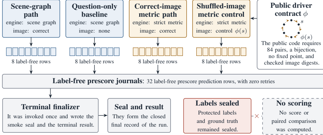
Figure 3: Four operational paths ran together in the V37 run. The paths were the scene-graph path, question-only baseline, correct-image metric path, and schema-matched shuffled-image metric control. Each path produced eight label-free prescore prediction rows, so the run wrote 32 rows with zero retries. The execution, warning-scan, restoration, cleanup, and terminal-seal gates passed. In the public driver, the shuffled-image mode swaps each attached image through a control mapping \phi . That mapping must hold 84 pairs, be a bijection, and have no fixed point, and the loader checks the digest of every source and control image. The terminal finalizer ran once and wrote the smoke seal and the terminal result. Protected labels and ground truth remained sealed, and no score or paired comparison was computed, so the run establishes operational integrity only. The run is private, and the public repository cannot reproduce it.
