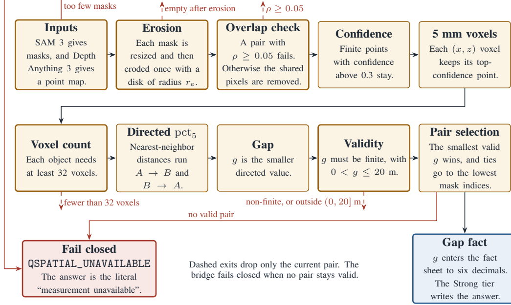
Figure 2: The strict metric bridge computes a horizontal gap from object masks and a point map. Each candidate pair of object masks passes through the steps from left to right, first along the top row and then along the bottom row. Here \text{pct}_5 is the fifth percentile with linear interpolation, as in Eq. (12). The erosion radius r_e is the ceiling of the larger resolution ratio between a mask and the point map. Each mask is first resized to the point-map grid by nearest-neighbor sampling. The overlap coefficient is \rho = |E_a \cap E_b| / \min(|E_a|, |E_b|) for the eroded masks E_a and E_b . The bridge returns QSPATIAL_UNAVAILABLE at once when the parser marks the question unsupported or when segmentation returns too few masks. A parse or manifest failure raises an error before the steps in this figure begin. Every dashed exit drops only the current pair, and the bridge returns QSPATIAL_UNAVAILABLE when no pair stays valid. The confidence filter has no exit of its own, because a mask that loses its points fails the voxel count. A segmentation or reconstruction service failure raises an error, and the bridge never falls back to the scene graph. A valid gap enters the fact sheet, and the Strong tier writes the final answer from it.
