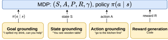
Figure 3: Grounding of MDP components through natural language. Each subcategory maps verbal feedback to a specific element of the MDP: goal grounding specifies the objective, state grounding represents observations as text, action grounding resolves instructions to executable behavior, and reward code generation compiles language into executable reward functions.
