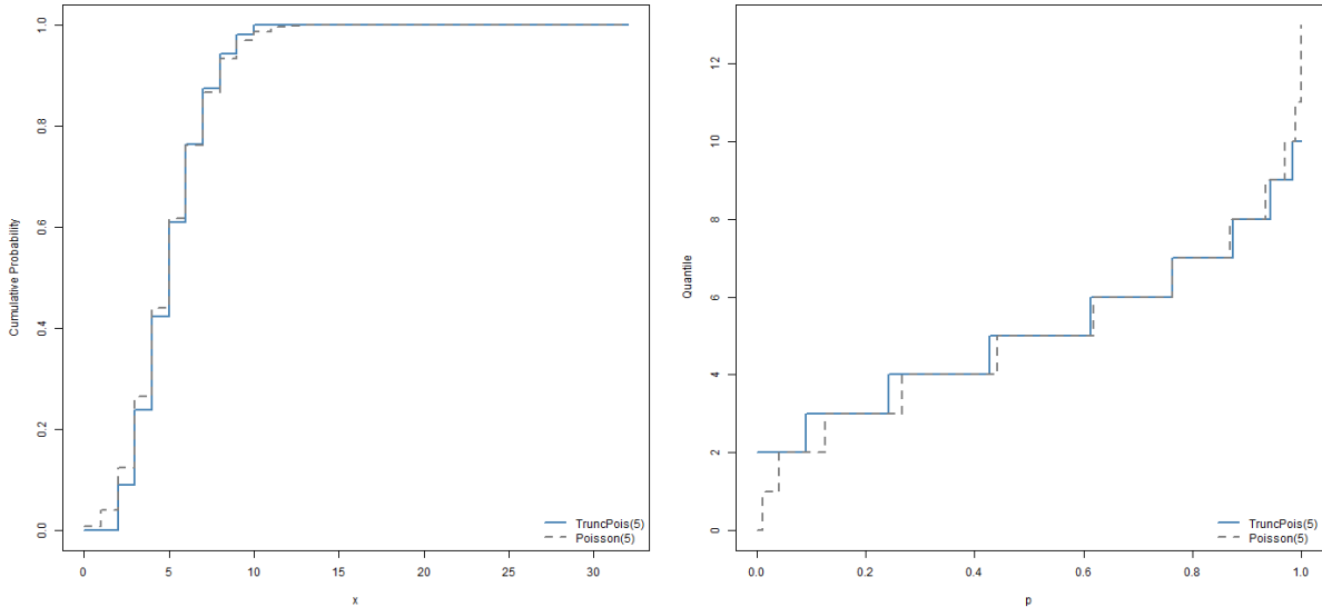
Figure 1: CDF and quantile function plots via plottruncpois() , comparing TruncPois( \lambda = 5 , a = 2 , b = 10 ) against Poisson( \lambda = 5 ) .
