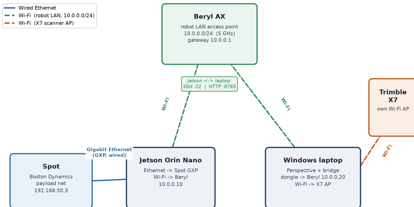
Field Network Topology - three non-overlapping subnets
