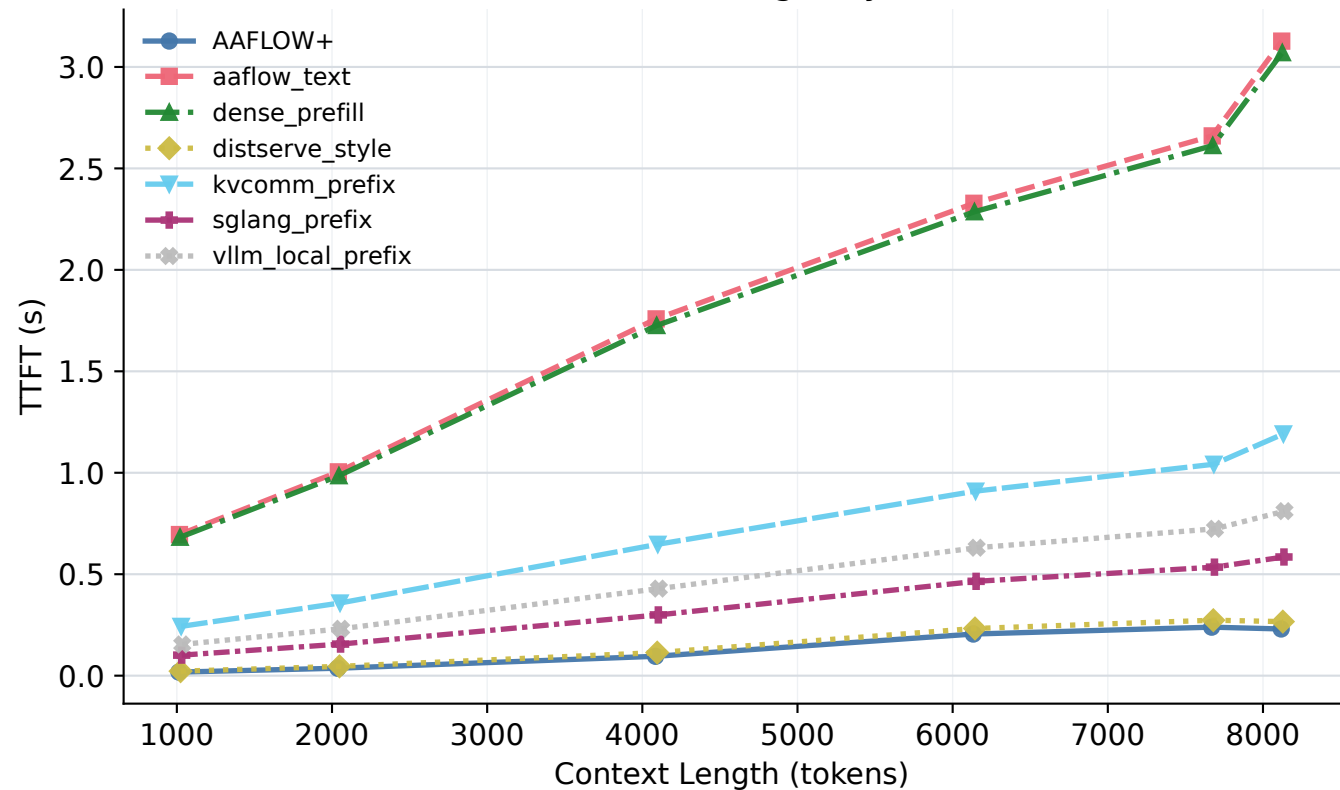
TTFT vs Context Length by Baseline
