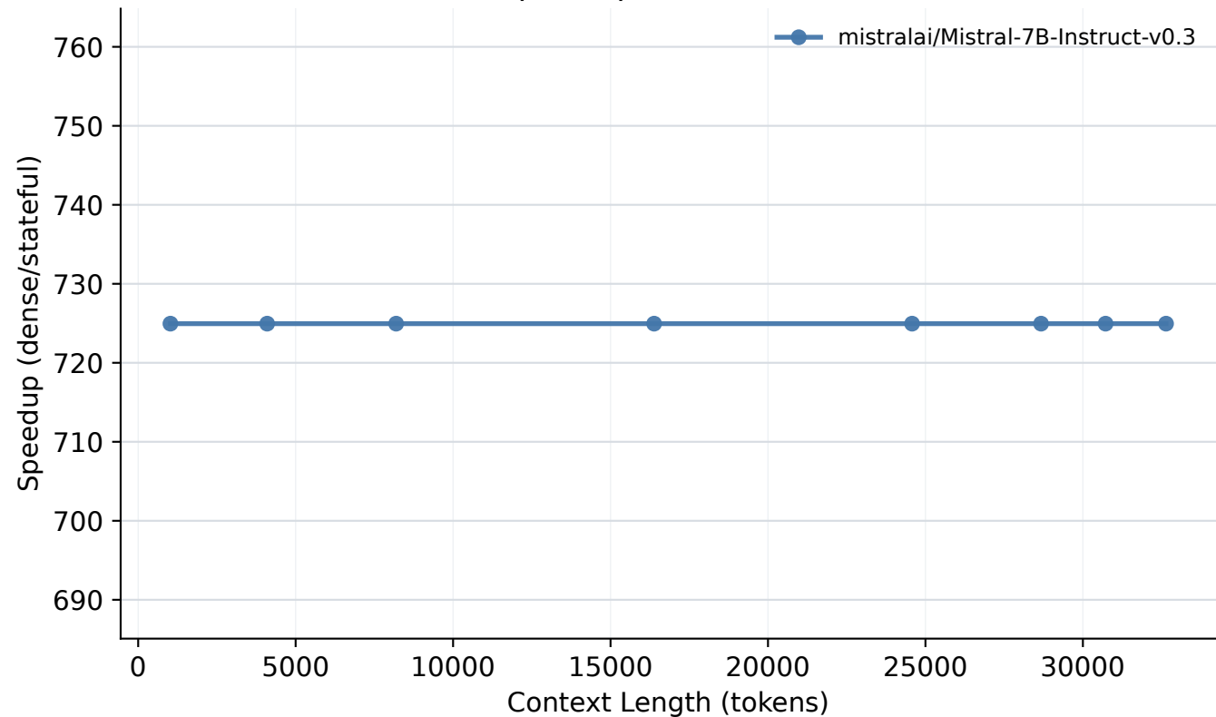
TTFT Speedup over Dense Prefill
