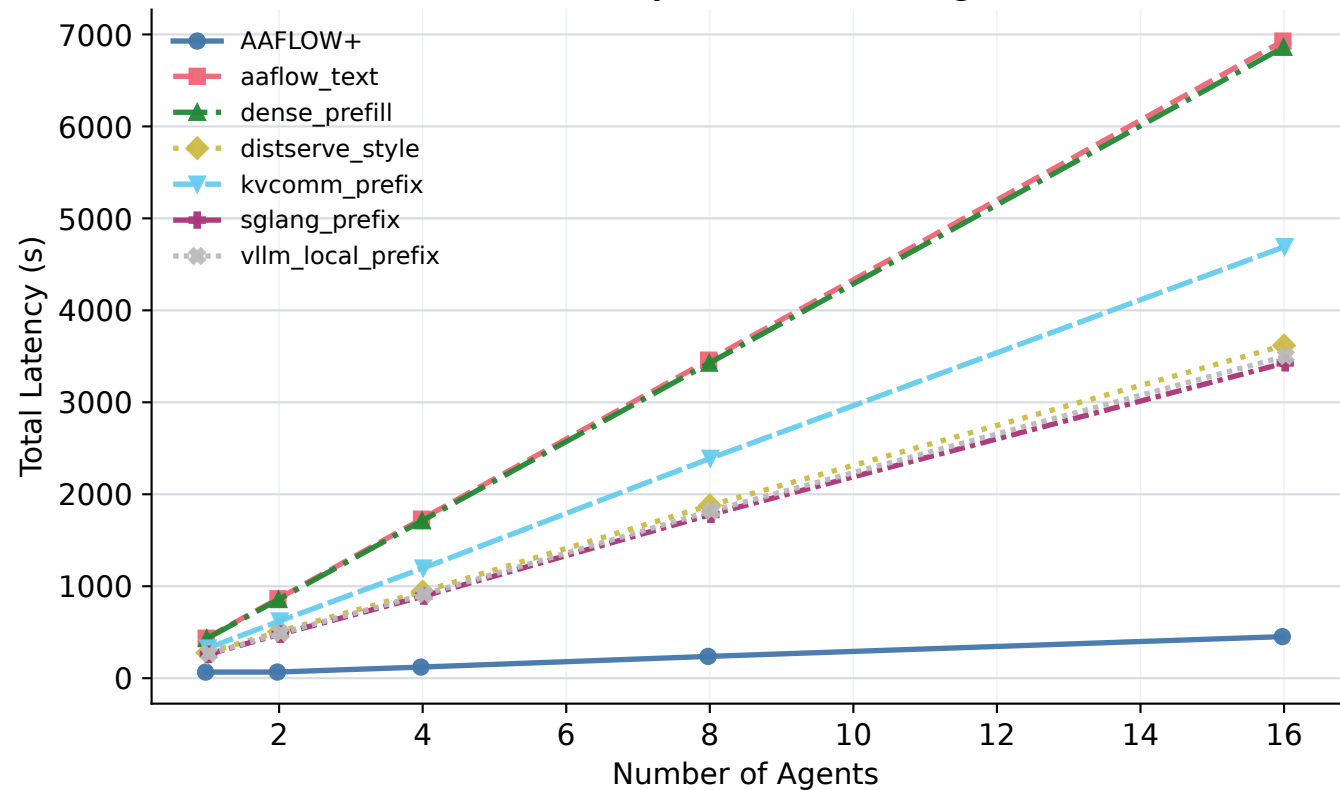
Total Latency vs Number of Agents
