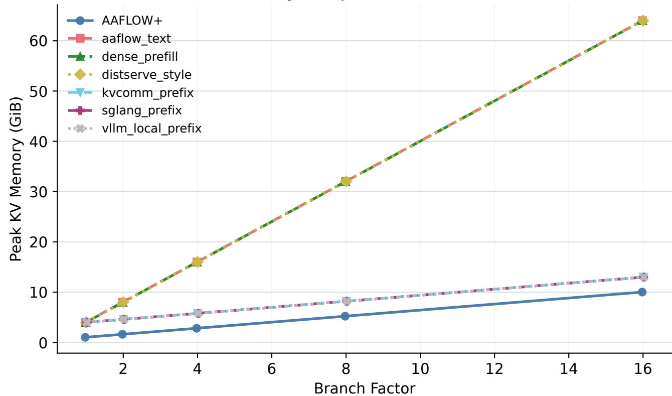
KV Memory Footprint vs Branch Factor
