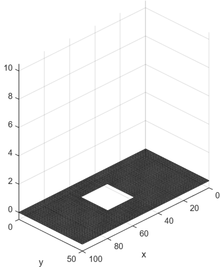
Density Surface ( \rho ) at t=0.00
