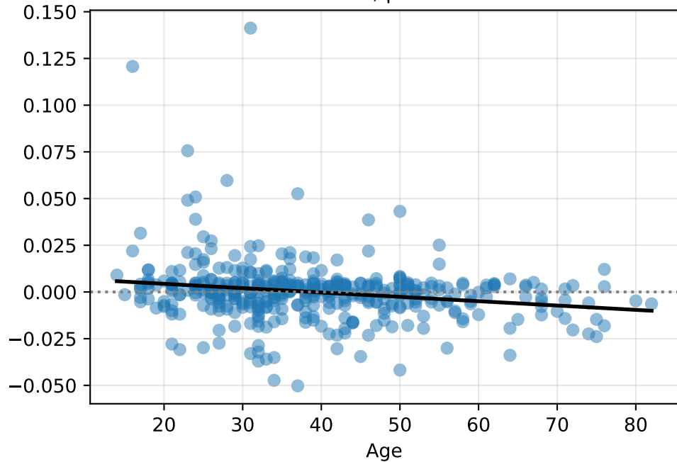
Fan improvement (W1→W3) r = -0.198, p < 0.0001
