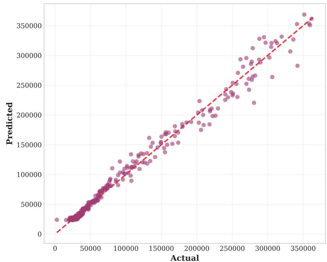
(c) Full Model Fit R^2 = 0.9860
