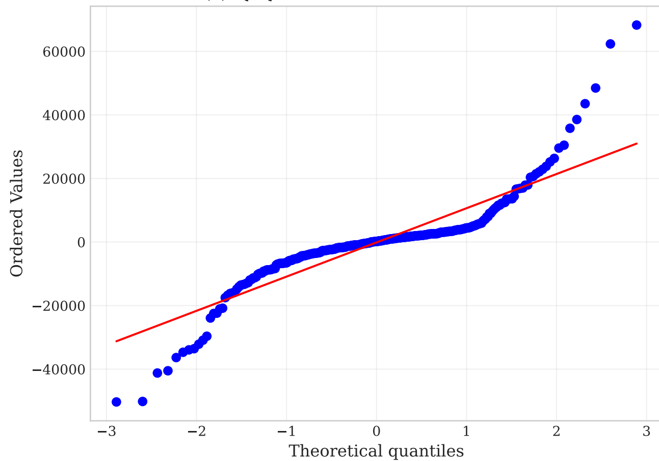
(c) Q-Q Plot: Base Model Residuals
