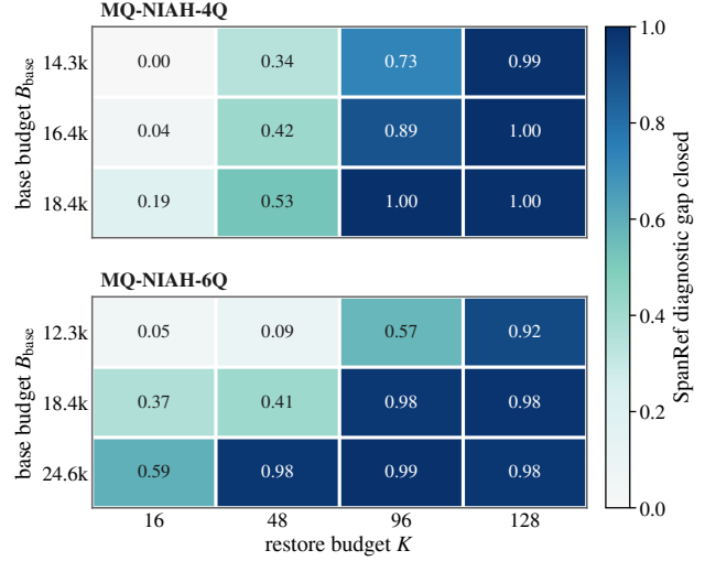
Figure 8. Operating regime: cells show the fraction of available SpanRef- K diagnostic gain recovered by REPAIRKV, clipped to [0, 1] , for MQ-NIAH-4Q/6Q. Saturated cells with little matched-to-SpanRef- K gap should not be read as upper-bound statements.
