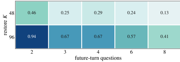
Figure 7. Query-count breadth: cells show REPAIRKV score gain over matched no-repair for K = 48 and K = 96 across 2-, 3-, 4-, 6-, and 8-question split-query variants.
