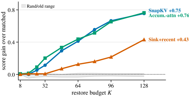
Figure 4. First-stage eviction-policy sensitivity on MQ-NIAH-4Q ( n=24 , B_{\text{base}}=16,384 ). Curves show exact Q_2 gain over each policy’s matched no-repair baseline. The gray band spans Random- K /Oldest- K gains.
