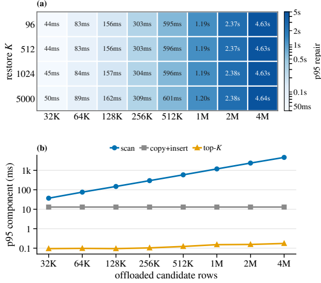
Figure 5. Runtime-capacity probe on the evaluation GPU. (a) Component-summed p95 service time for chunked scan, top- K selection, and KV movement at query length 64 over pinned host-memory BF16 KV-shaped tensors. (b) Stage-wise p95 component time for K = 5000 . Generation and answer evaluation are excluded.
