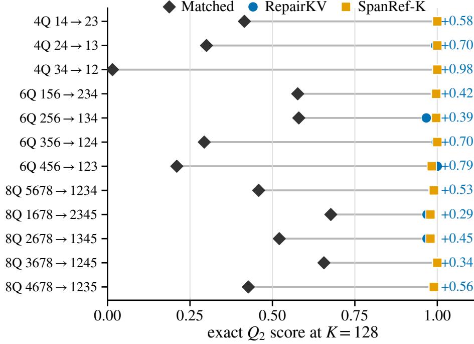
Figure 8. Per-partition endpoint scores at K = 128 on the final exact evaluations. Gray segments show the change from matched no-repair to REPAIRKV, orange points show the benchmark-metadata SpanRef- K diagnostic, and labels report the REPAIRKV difference over matched no-repair.
