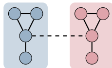
Two identified communities
