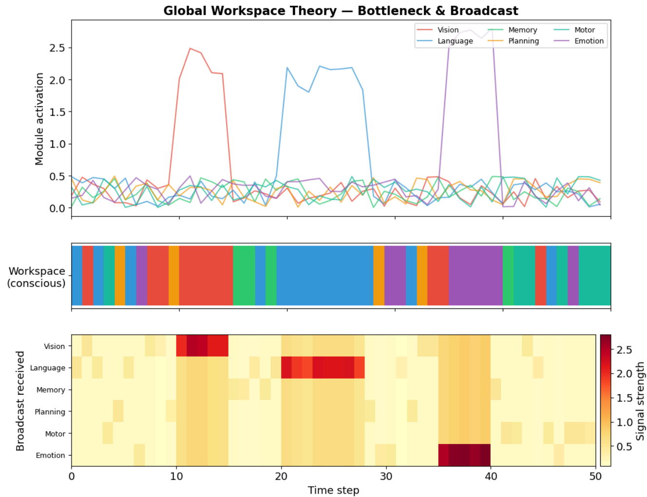
Figure 3. Simulation of Global Workspace Theory (Baars, 1988). Top: six specialized modules compete for access to a shared workspace. Middle: the workspace bottleneck — only the most active module "wins" at each time step (color = winning module). Bottom: the broadcast pattern — when a module enters the workspace, its signal is broadcast to all other modules, modeling consciousness as selective, competitive broadcasting.
