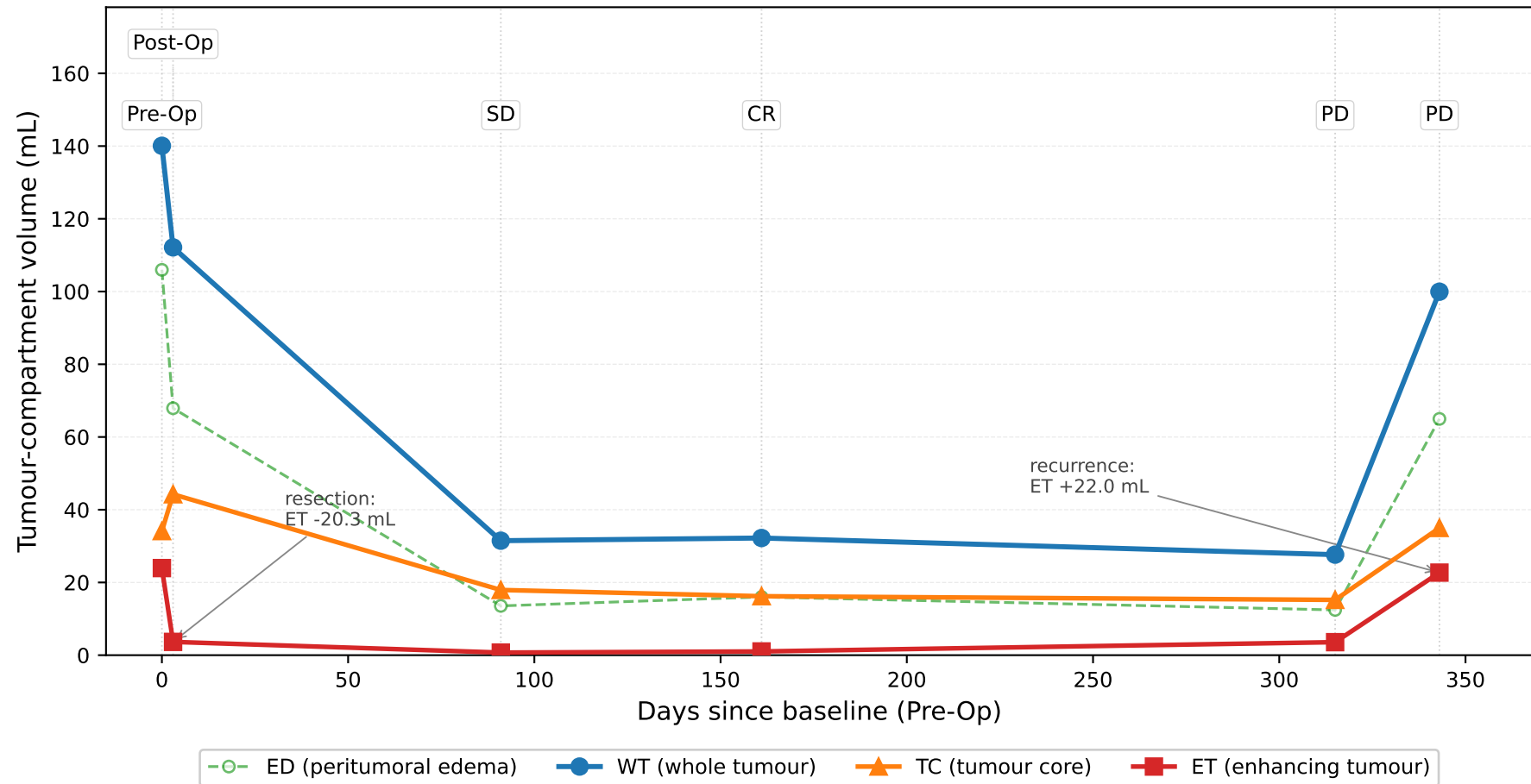
LUMIERE Patient-048 -- longitudinal tumour volumes (unified MONAI Bundle BraTS three-class SegResNet, n = 6 timepoints)
