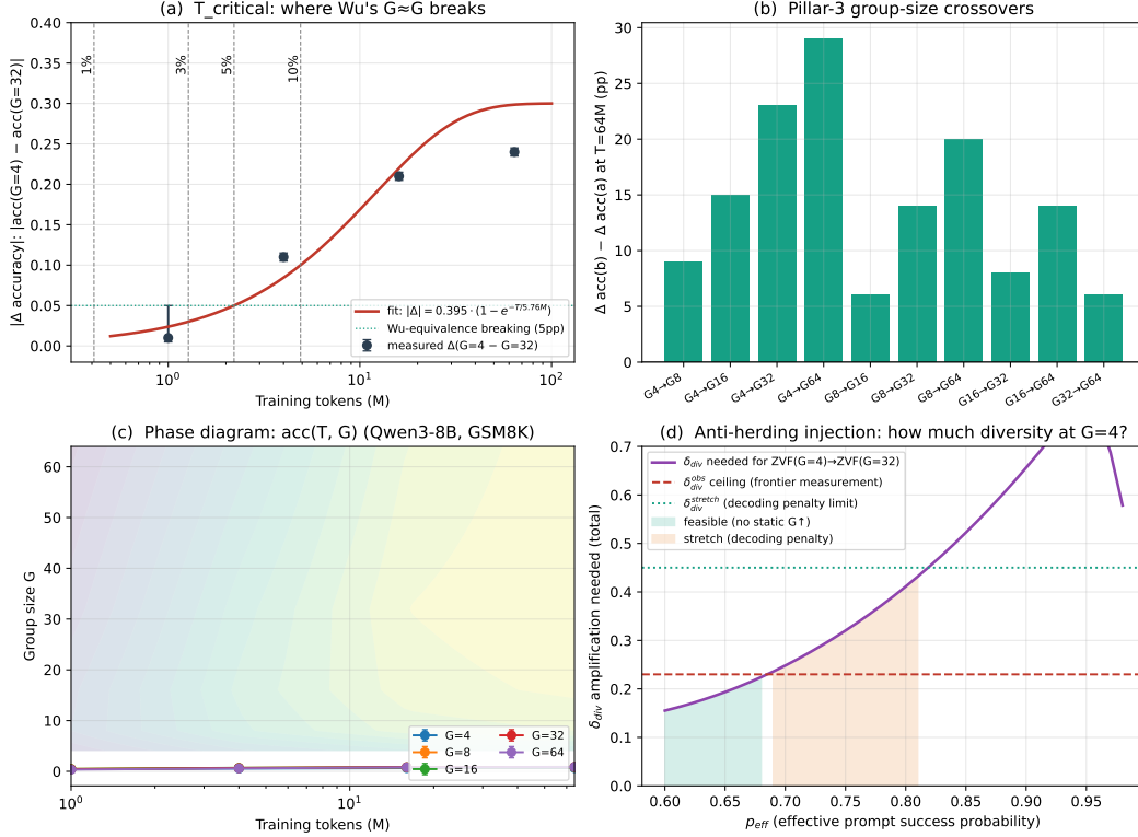
Figure 11: Pillar-3 elevation panel. (a) |\Delta(G=4-G=32)| vs. training tokens (paired bootstrap); the dashed vertical lines mark T_{\text{crit}}^{1\%} = 0.41M , T_{\text{crit}}^{3\%} = 1.27M , T_{\text{crit}}^{5\%} = 2.21M , T_{\text{crit}}^{10\%} = 4.91M . (b) Per-pair \Delta_{\text{pp}} at T=64M tokens; positive bars mark pairs where the larger G_b wins ( frontier synthesis ). (c) \text{acc}(T, G) phase diagram on Qwen3-8B / GSM8K; iso-acc contours from the dense grid. (d) \delta_{\text{div}} amplification required for ZVF( G=4 ) \rightarrow ZVF( G=32 ) vs. p_{\text{eff}} , with the \delta_{\text{div}} \leq 0.23 natural ceiling and the \delta_{\text{div}} \leq 0.45 stretch (decoding penalty) limits.
