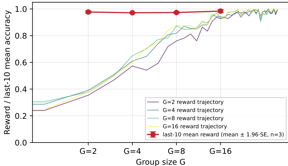
Reward vs G on measured Qwen2.5-0.5B / arithmetic (40 steps × 3 seeds, near-ceiling task)
