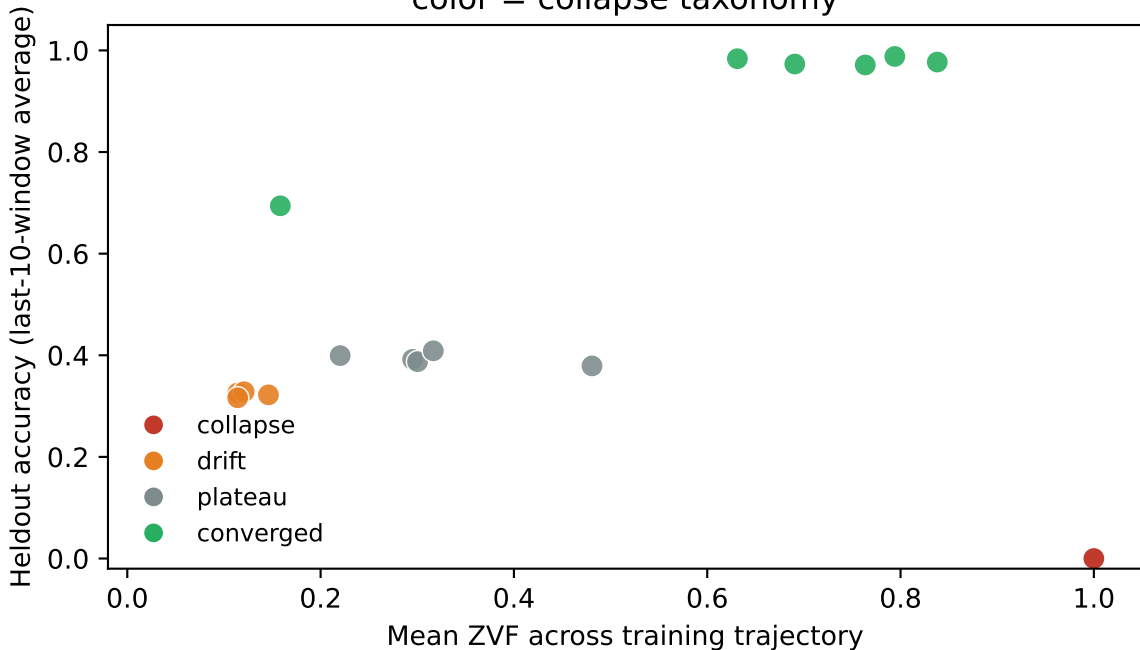
ZVF vs training outcome across 17 (experiment, model, G) cells color = collapse taxonomy
