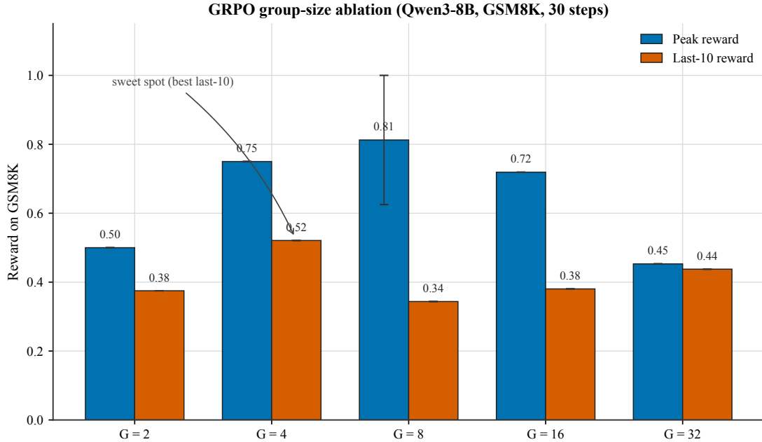
Figure 17: Empirical GRPO group-size ablation on Qwen3-8B / GSM8K (30 training steps, G \in \{2, 4, 8, 16, 32\} ). Blue bars show peak reward during training; vermilion bars show last-10 average reward, aggregated across the campaign_v2_w2_* , campaign_v2_w1_qwen3-8b-base , and scale_gsm8k_qwen3-8b seeds (for G=8 ). Although peak reward rises monotonically up to G=8 (0.50, 0.75, 0.81, 0.72, 0.45), the last-10 average peaks at G=4 (0.52). We annotate G=4 as the empirical sweet spot : higher group sizes trade per-step variance reduction for end-of-training stability.
