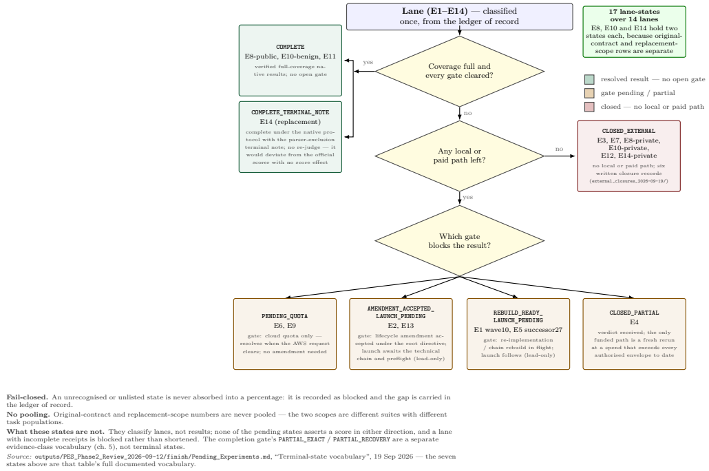
Figure 9.5: Terminal-state taxonomy used to close every lane. Each state has a defined meaning and a named reopen condition where one exists.
