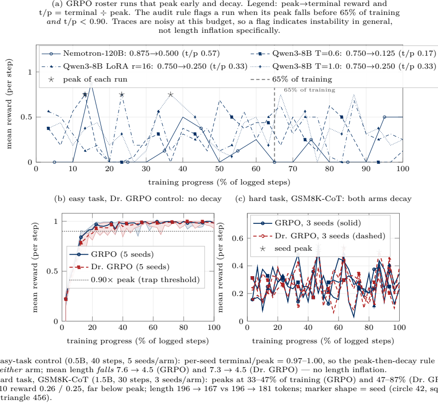
Figure 6.4: Roster-level reward trajectories. Four of eleven GRPO runs carry the post-hoc verbosity-trap flag (peak before 65% of training, terminal reward below 90% of peak). The flag tests in-training reward, not length, so it is a description of the roster and not evidence of length bias; the controlled sixteen-run comparison shows no flags.
