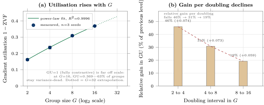
Figure 4.5: Gradient utilisation, 1 - \text{ZVF} , as a function of group size G . Increasing G reduces the zero-variance fraction with saturating benefit, which is why larger groups are not uniformly better.
