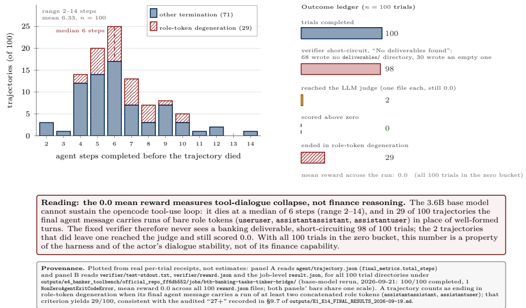
Figure 9.4: The E4 rerun diagnostic. Across 100 trials agents terminate at a median of roughly six steps without producing deliverables, and more than a quarter end in role-token degeneration. The 0.0 mean reward therefore measures tool-dialogue collapse, not finance reasoning.
