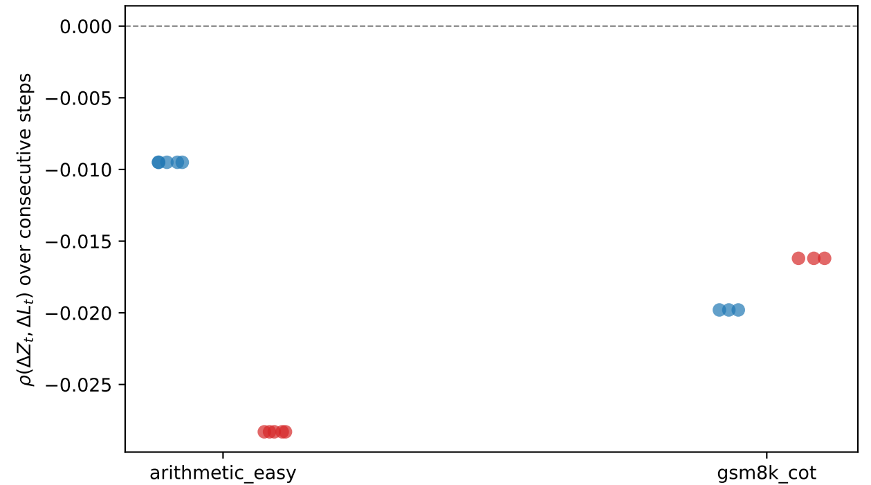
D. H4 ZVF-length co-movement; >0 = ZVF falls with length shrink
