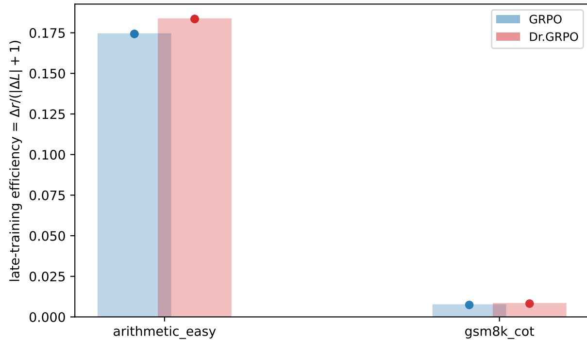
C. H3 late-training efficiency (GR blue, Dr.GR red); dots = seeds
