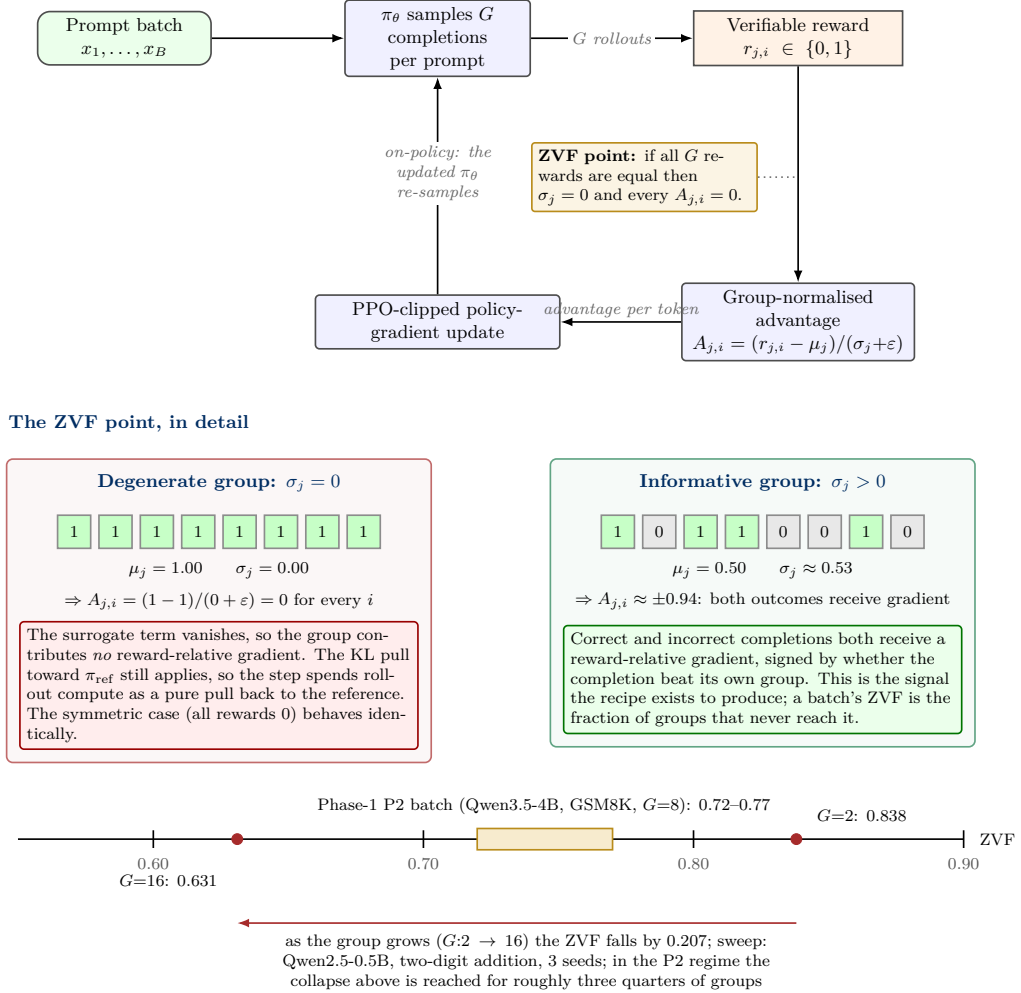
Figure 1.1: The GRPO training loop. A prompt is sampled G times, each completion is scored by a reward function, advantages are formed relative to the group, and the policy is updated. When all G rewards coincide the group-relative advantage collapses to zero and no reward-relative gradient flows, although the rollouts are still paid for. Number line: the Phase-1 P2 batch ZVF of 0.72–0.77 (four methods, 40 steps, 16 prompts \times 8 samples, GSM8K, seed 0, Qwen3.5-4B) and the group-size sweep on Qwen2.5-0.5B two-digit addition over three seeds, where mean ZVF falls from 0.838 at G = 2 to 0.631 at G = 16 (a fall of 0.207).
