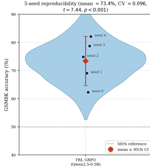
Figure 19: Cross-seed reproducibility analysis for TRL GRPO on Qwen2.5-0.5B (GSM8K, 125 steps, NVIDIA L4). Five seeds show mean accuracy 73.4% with CV = 0.096. Violin plot shows the distribution; individual seeds are labeled. The mean is significantly above 50% ( t = 7.44 , p < 0.001 ), confirming that GRPO produces reliable learning signal even at 0.5B scale.
