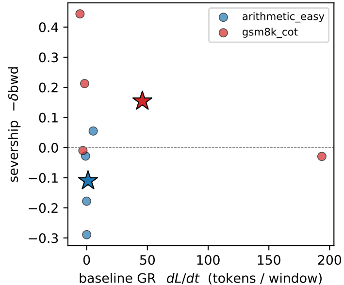
(A) sever vs baseline dL/dt
