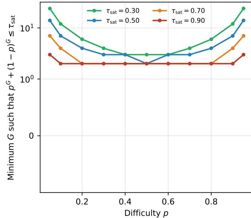
(c) Iso-G saturation floor
