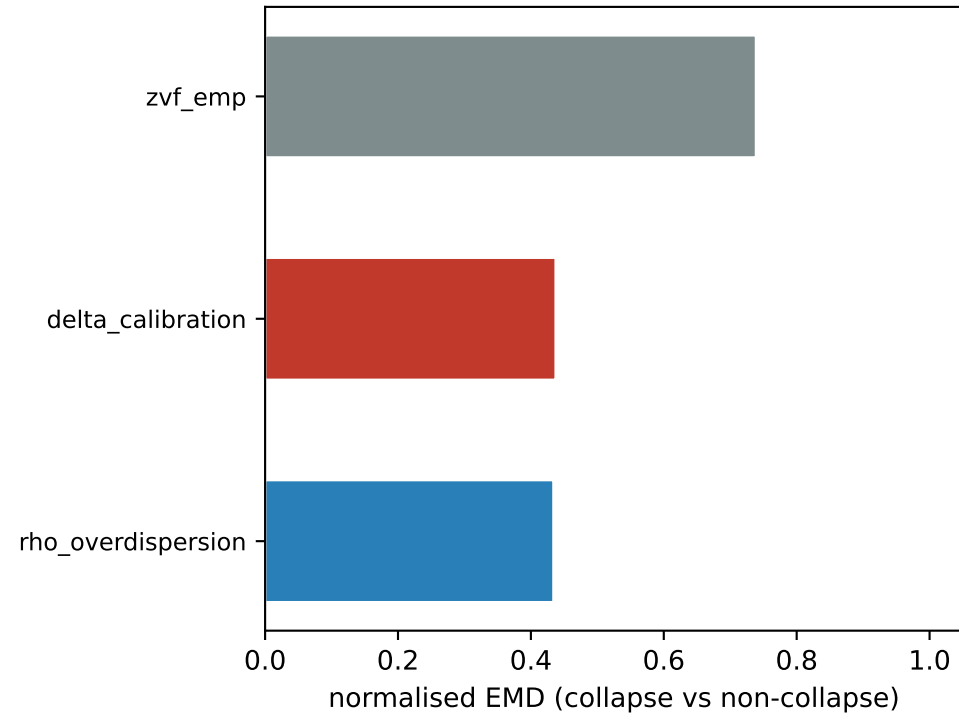
(b) 1-Wasserstein separation
