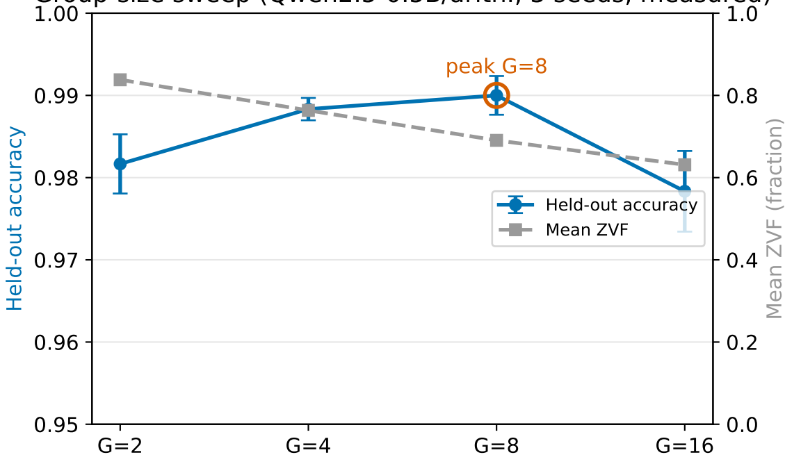
Group-size sweep (Qwen2.5-0.5B/arith., 3 seeds, measured)
