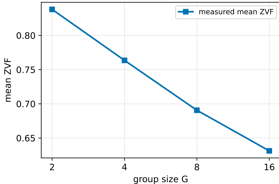
ZVF decreases with G (Qwen2.5-0.5B/arith., measured)
