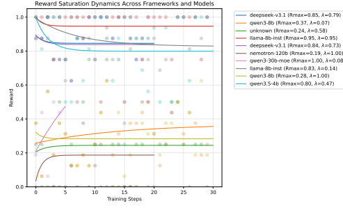
Figure 20: Exponential saturation curve fitting across models ( R_{max} and \lambda ). Legacy baselines fail to saturate.
