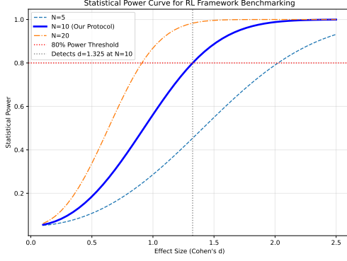
Figure 19: Statistical power analysis demonstrating that N = 10 provides 80% power to detect d = 1.325 .
