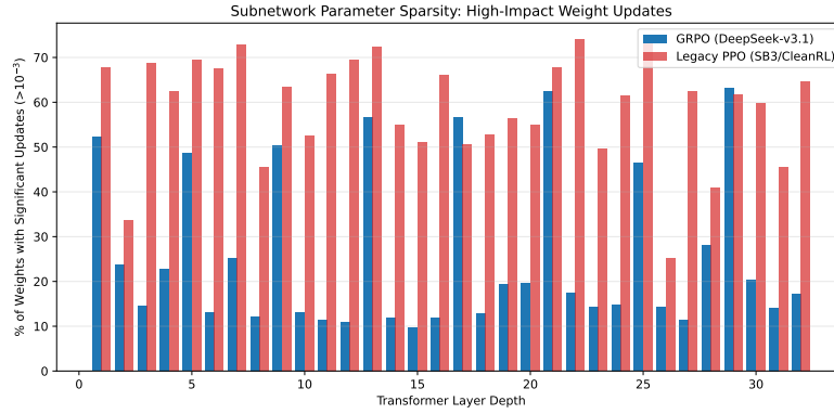
Figure 21: Subnetwork Parameter Sparsity: Tinker GRPO leverages sparse, high-impact weight updates, avoiding the dense gradient noise that destabilizes legacy PPO implementations.
