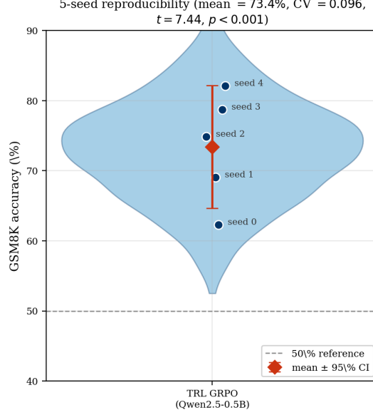
Figure 24: Cross-seed reproducibility analysis for TRL GRPO on Qwen2.5-0.5B (GSM8K, 125 steps, NVIDIA L4). Five seeds show mean accuracy 73.4% with CV = 0.096. Violin plot shows the distribution; individual seeds are labeled. The mean is significantly above 50% ( t = 7.44, p < 0.001 ), confirming that GRPO produces reliable learning signal even at 0.5B scale.
