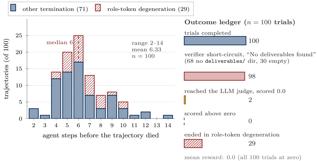
Figure 9.5: The E4 rerun diagnostic. Across 100 trials agents terminate at a median of roughly six steps without producing deliverables, and more than a quarter end in role-token degeneration, consistent with generation running past the end-of-turn token because the serving bridge passed no stop sequences. The 0.0 is not a measurement of finance reasoning. Left: per-trajectory step counts ( final_metrics.total_steps ), stacked by whether the final agent message carries at least two concatenated role tokens (29/100; the ledger records “27+”). Right: where the verifier chain stopped ( verifier/test-stdout.txt , reward.json ), all bars on one scale. Base-model rerun of 2026-09-21, all 100 trial directories under outputs/e4_banker_toolbench/ .
