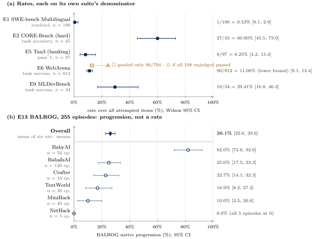
Figure 9.4: The six replacement-scope results scored on 2026-09-27, each with its 95% confidence interval. (a) Rates over all attempted items, with errors, timeouts and ungraded items counted as failures (Wilson intervals). For E6 WebArena the filled point is the lower bound 90/812; the square is the rate over the 704 judged tasks and the triangle the value if all 108 unjudged tasks had passed. (b) E13 BALROG reports native progression, not a success rate: per-environment means with percentile-bootstrap intervals ( B = 10,000 ), and the BALROG overall score, the unweighted mean of the six environment means, with its normal-approximation interval. Each row is a different suite with its own metric and denominator, so no cross-lane average is drawn, and none of these values is pooled with an original-contract figure. Source: outputs/finish_pending_2026-09-27/<lane>/result.json .
