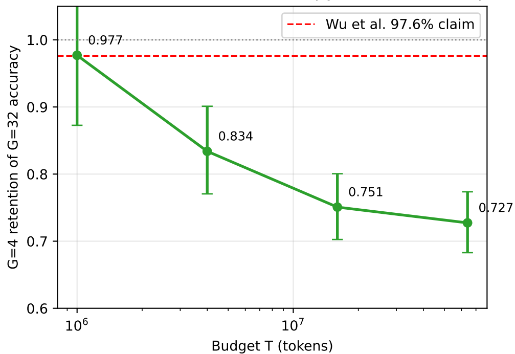
B. Broader-scale G=4 ~ G=32 (Qwen3-8B / GSM8K)
