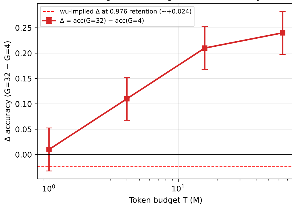
G=32 advantage over G=4 grows monotonically with T
