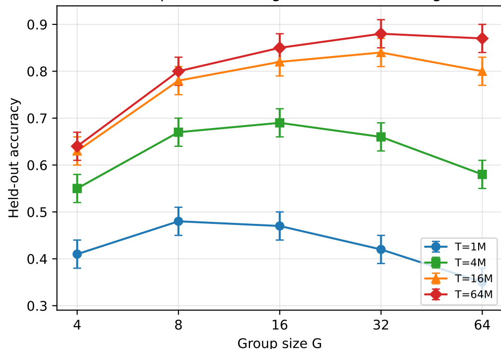
Acc vs G per token budget (crossover at large T)
