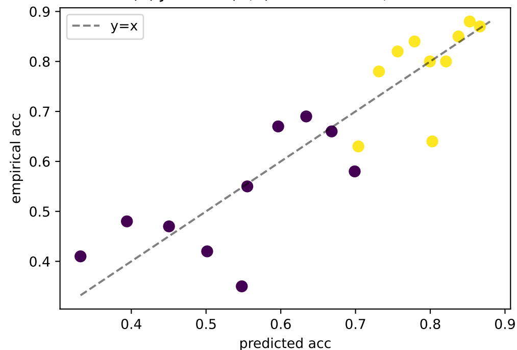
(A) Joint acc(G,T) fit: R^2=0.796 , n=20
