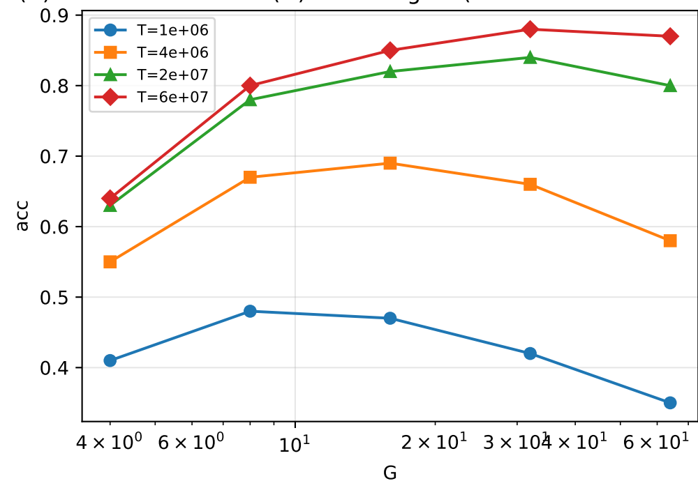
(C) Bounded cone: acc(G) at 4 budgets ( G=64 \leq G=32 at every T)
