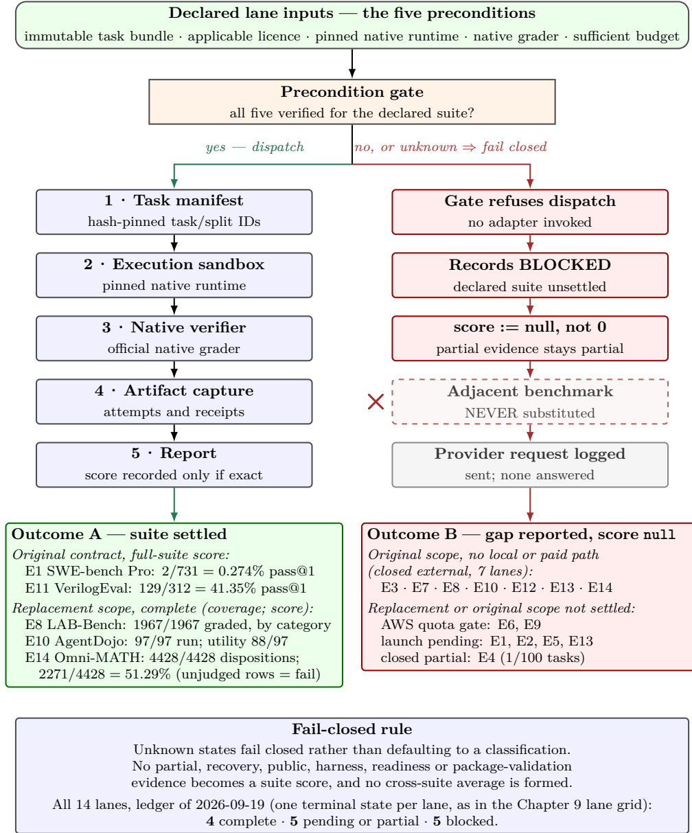
Figure 5.3: Evaluation harness internals. The harness is fail-closed: when a precondition cannot be satisfied the lane records BLOCKED rather than substituting an adjacent benchmark. Outcomes and the lane tally are taken from the 2026-09-19 ledger of record (Pending_Experiments.md). Outcome A separates original-contract scores from replacement-scope results and gives coverage and score separately; Outcome B lists original-scope suites that are closed external, then lanes whose scope is not yet settled. E14 is reported as 2271/4428 = 51.29% with the two unjudged rows counted as failures (the official scorer reports 51.31% over 4426 judged rows).
