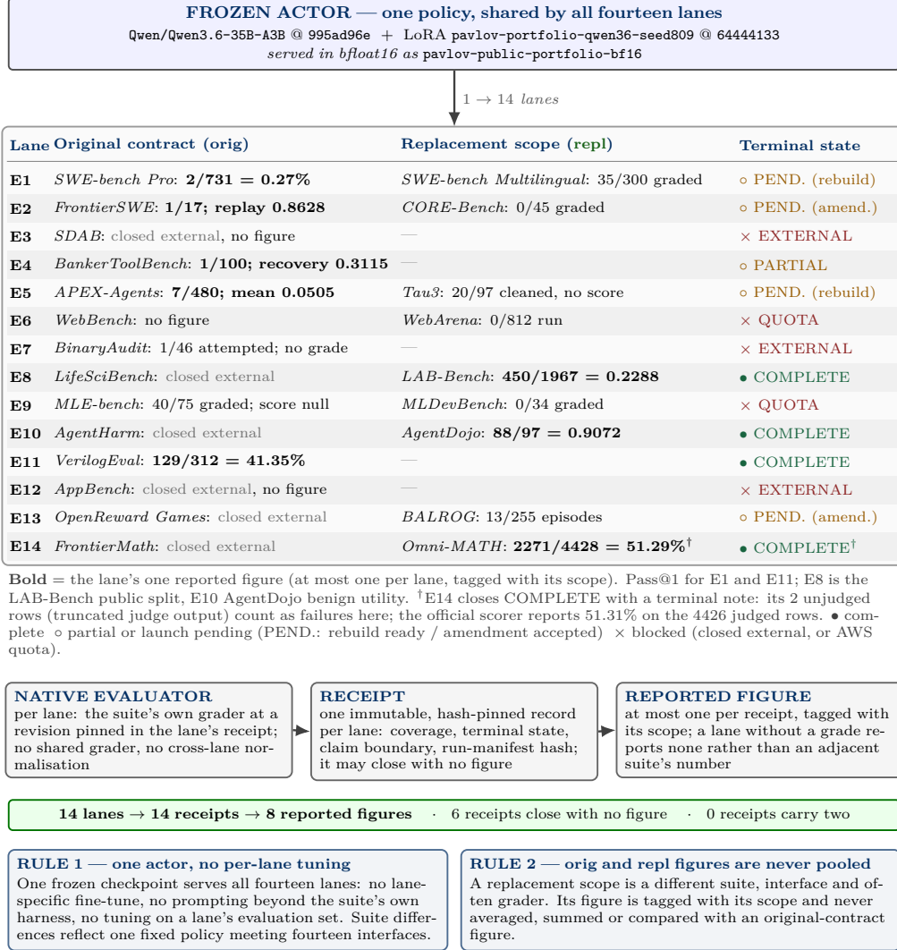
Figure 4.6: Design of the E1–E14 held-out evaluation campaign. One frozen actor serves all fourteen lanes, and each suite is graded by its own native evaluator at a pinned revision. Each lane lists its original-contract suite and, where one exists, its replacement scope side by side; Figure 9.1 names the replacement scope where one exists. Figures and terminal states come from the 2026-09-19 ledger (E1_E14_FINAL_RESULTS_2026-09-19.md and finish/Pending_Experiments.md; 11/11 deterministic checks pass). E14’s 2271/4428 = 51.29% counts the 2 unjudged rows as failures; the official scorer reports 51.31% = 2271/4426 on the judged rows.
