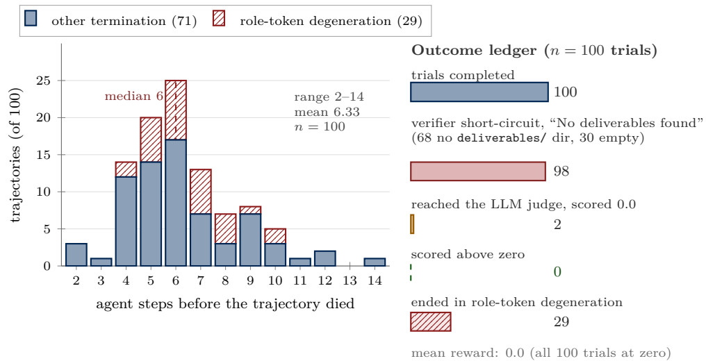
Figure 9.4: The E4 rerun diagnostic. Across 100 trials agents terminate at a median of roughly six steps without producing deliverables, and more than a quarter end in role-token degeneration, consistent with generation running past the end-of-turn token because the serving bridge passed no stop sequences. The 0.0 is not a measurement of finance reasoning. Left: per-trajectory step counts ( final_metrics.total_steps ), stacked by whether the final agent message carries at least two concatenated role tokens (29/100; the ledger records “27+”). Right: where the verifier chain stopped ( verifier/test-stdout.txt , reward.json ), all bars on one scale. Base-model rerun of 2026-09-21, all 100 trial directories under outputs/e4_banker_toolbench/ .
