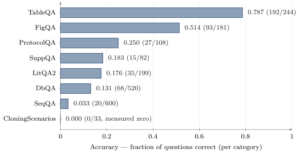
Figure 9.2: LAB-Bench public split, per-category accuracy, all 1,967 questions graded across eight categories. Each bar is correct/total for one category (labels give the counts). Accuracy is strongly category-dependent, so no pooled cross-category average is drawn or claimed. CloningScenarios is a measured zero (0/33), not a missing value.
