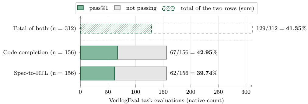
Figure 9.3: VerilogEval decomposition: two native framings of 156 tasks, 67/156 code-completion and 62/156 spec-to-RTL, summing to 129/312 = 41.35% pass@1. The dashed top bar is the sum of the two rows, not a third measurement. Graded by the suite's native harness (receipt e11_full_receipt.json); the 129/311 = 41.48% value that excludes Prob099_m2014_q6c is a non-canonical sensitivity only.
