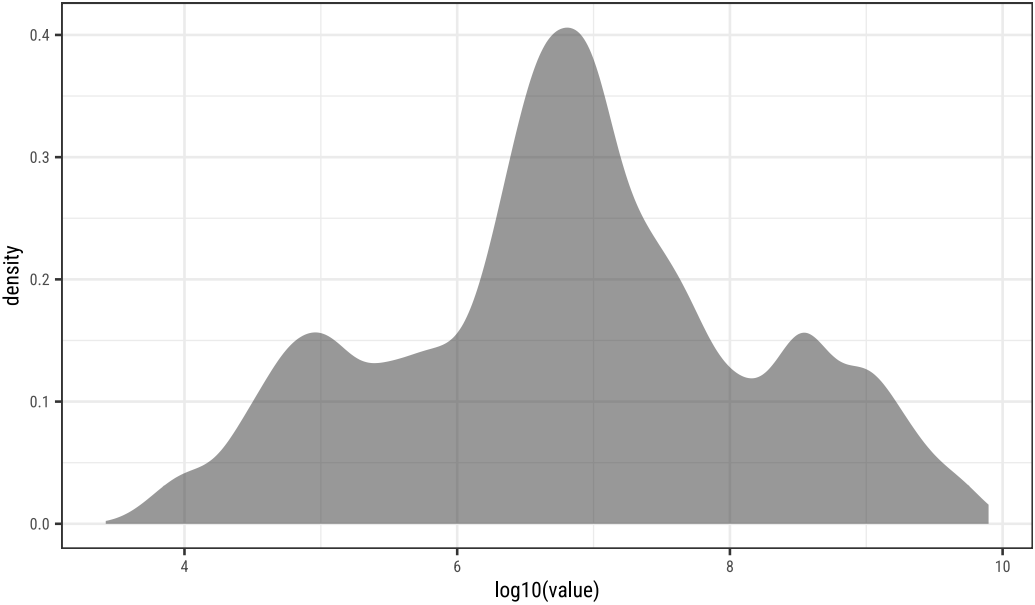
Density with Log transformed x-variable
