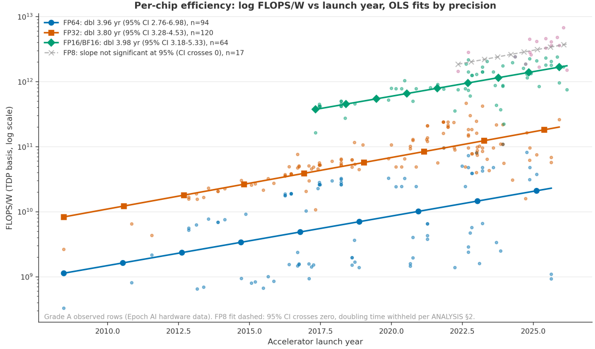
Figure 2: Per-chip efficiency: log FLOPS/W (TDP basis) vs. accelerator launch year, with OLS fits of \ln(\text{value}) on launch year per precision (Epoch AI machine-learning-hardware data, all grade A observed rows). FP64 ( hw-flops-per-watt-fp64 , n = 94 , 2008-06-16 to 2025-08-22): doubling 3.96 yr (95% CI 2.76–6.98); FP32 ( hw-flops-per-watt-fp32 , n = 120 , 2008-06-16 to 2025-12-02): 3.80 yr (3.28–4.53); FP16/BF16 ( hw-flops-per-watt-fp16bf16 , n = 64 , 2017-05-01 to 2026-03-11): 3.98 yr (3.18–5.33); FP8 ( hw-flops-per-watt-fp8 , n = 17 , 2022-05-10 to 2026-03-11): slope 0.186/yr with 95% CI (−0.020, 0.392) crossing zero: not significant at 95%, drawn dashed gray with the doubling time withheld per the analysis. Estimates: eff_fp64_watt_doubling_time , eff_fp32_watt_doubling_time , eff_fp16bf16_watt_doubling_time , eff_fp8_watt_doubling_time . Caveats: per-chip TDP (vendor thermal design power), not measured sustained draw; precisions never mixed; fit slopes re-verified in-script against key_estimates.csv before plotting.
