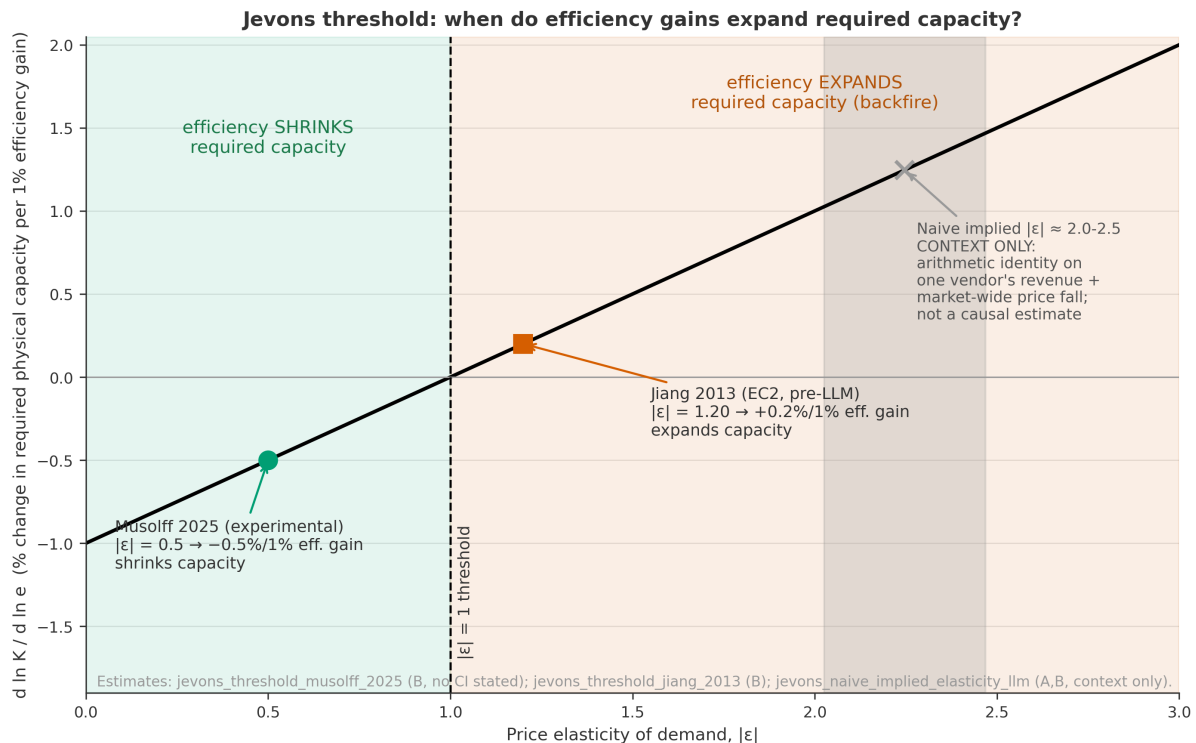
Figure 4: Jevons threshold diagram: d \ln K / d \ln e = |\varepsilon| - 1 vs. price elasticity of demand |\varepsilon| , where K is required physical capacity and e is efficiency (a 1% efficiency gain changes required capacity by (|\varepsilon| - 1)\% ). Green region ( |\varepsilon| < 1 ): efficiency shrinks required capacity; orange region ( |\varepsilon| > 1 ): backfire. Marked: Musolff 2025 experimental estimate |\varepsilon| = 0.5 \rightarrow -0.5\%/1\% gain (jeavons_threshold_musolff_2025, grade B; no numeric CI stated; cloud spot compute, not genAI inference); Jiang 2013 EC2 |\varepsilon| = 1.20 \rightarrow +0.2\%/1\% gain (jeavons_threshold_jiang_2013, grade B, pre-LLM era); |\varepsilon| = 1 threshold (dashed). Gray band: the naive arithmetic implied |\varepsilon| \approx 2.0-2.5 (jeavons_naive_implied_elasticity_llm = 2.247, CI 2.026–2.468), shown as context only: it mixes one vendor’s revenue growth with a market-wide price fall and is not a causal estimate.
