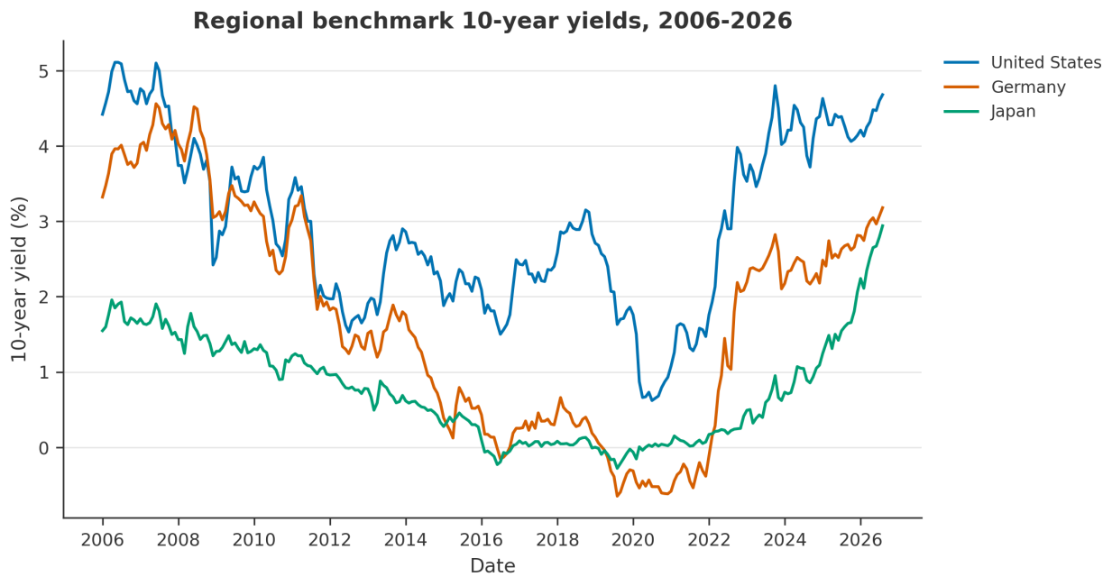
Figure 4: Regional benchmark 10-year yields, 2006-2026. The normalization of Japanese yields after 2022 mechanically compressed Asia-Pacific spreads.
