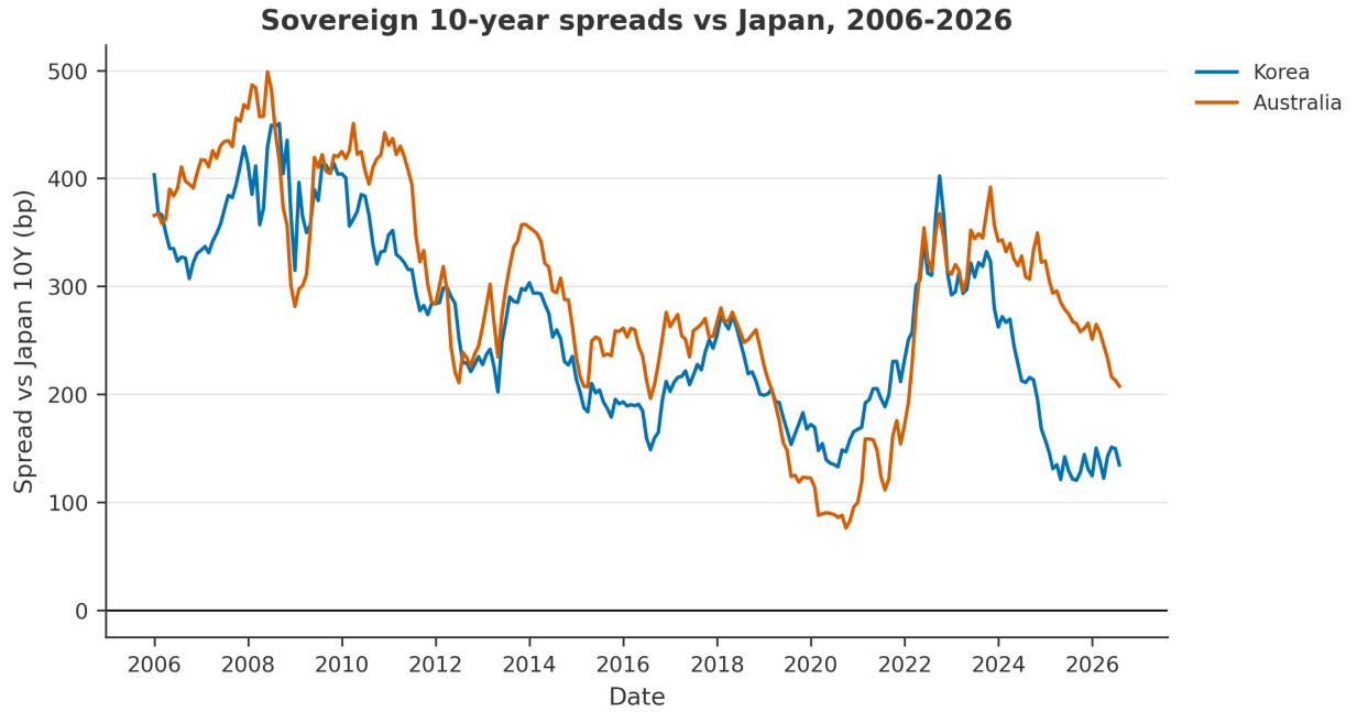
Figure 3: Monthly 10-year sovereign spreads vs Japan, 2006-2026. Korea and Australia.
