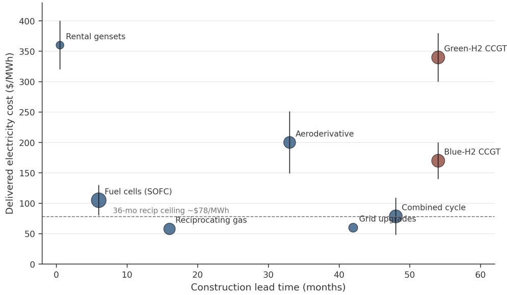
Figure 3: Alternatives by delivered electricity cost against construction lead time. Circle area scales with capex per kW. Only alternatives priced near grid power can clear the market for speed; hydrogen chains are a decarbonization option, not a time-to-power option.
