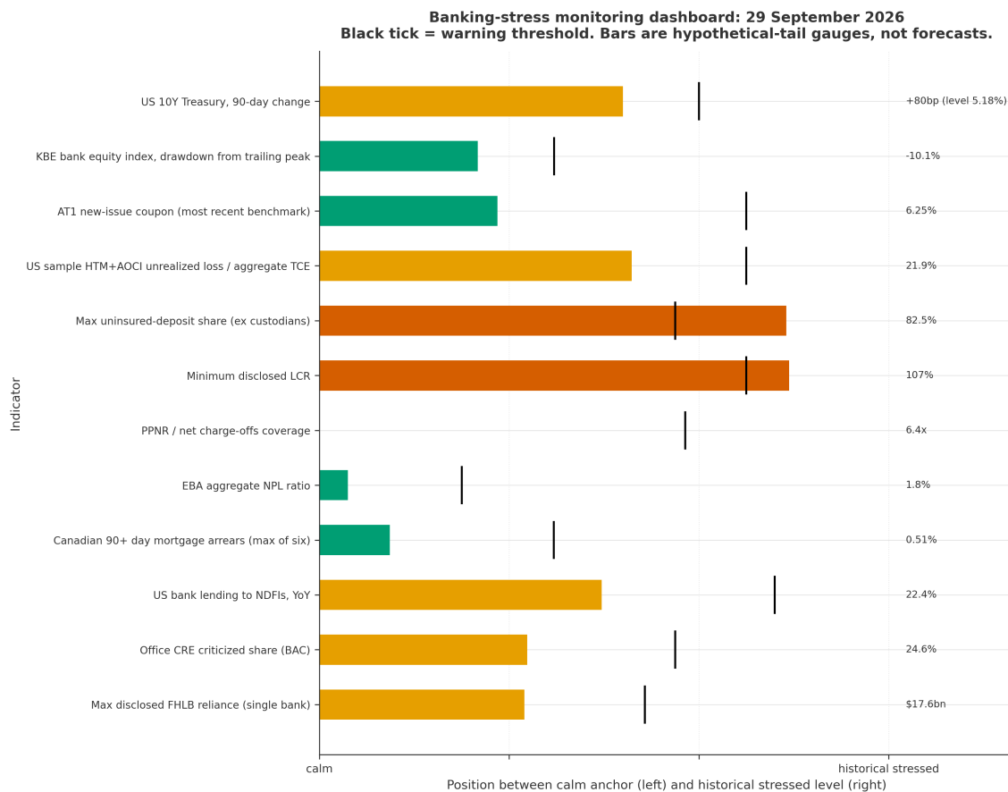
Figure 10. Banking-stress monitoring dashboard: current readings against warning thresholds (black ticks) on gauges from calm (left) to historical stressed levels (right). No indicator is at its historical stressed level; two sit at or past warning; two are within one move.
