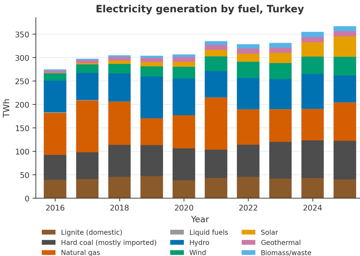
Figure 1. Electricity generation by fuel, Turkey, 2016–2025 (TWh)
