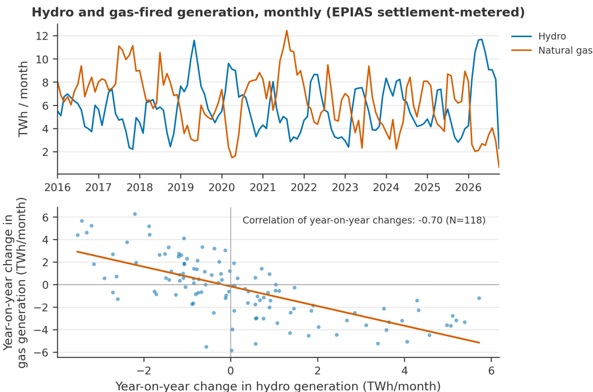
Figure 9. Hydro and gas-fired generation, monthly, Turkey (EPIAS settlement-metered, TWh/month, top); year-on-year monthly changes with fitted line (bottom), January 2016–October 2026
