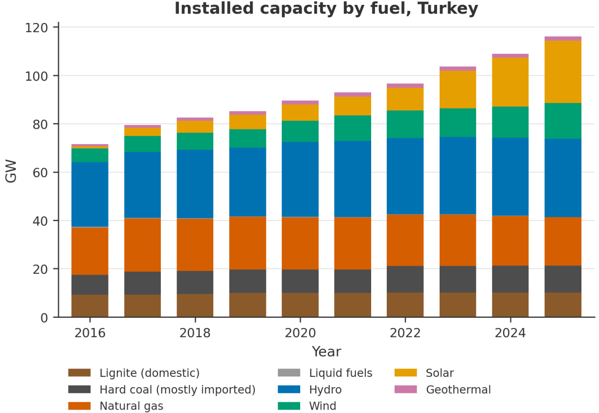
Figure 3. Installed capacity by fuel, Turkey, end-2016 to end-2025 (GW)
