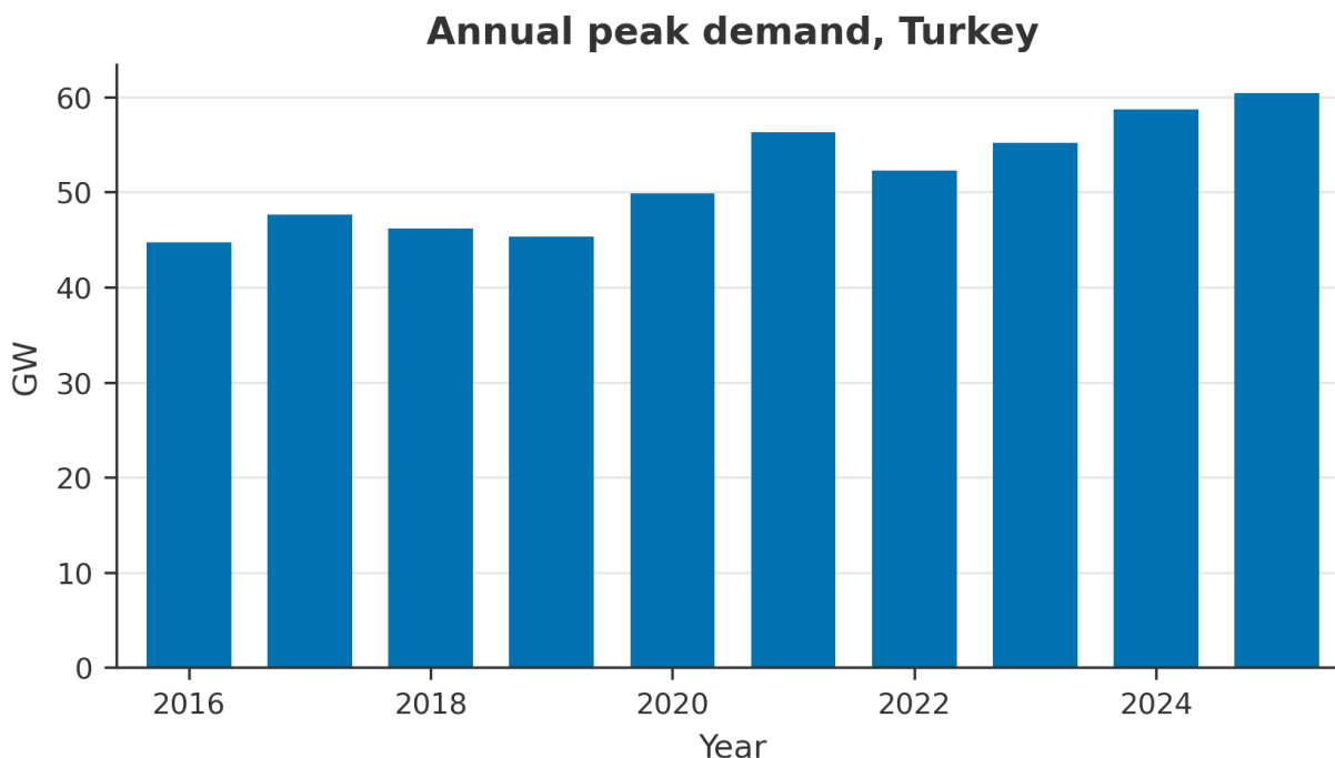
Figure 12. Peak demand, Turkey, 2016–2025 (GW)
