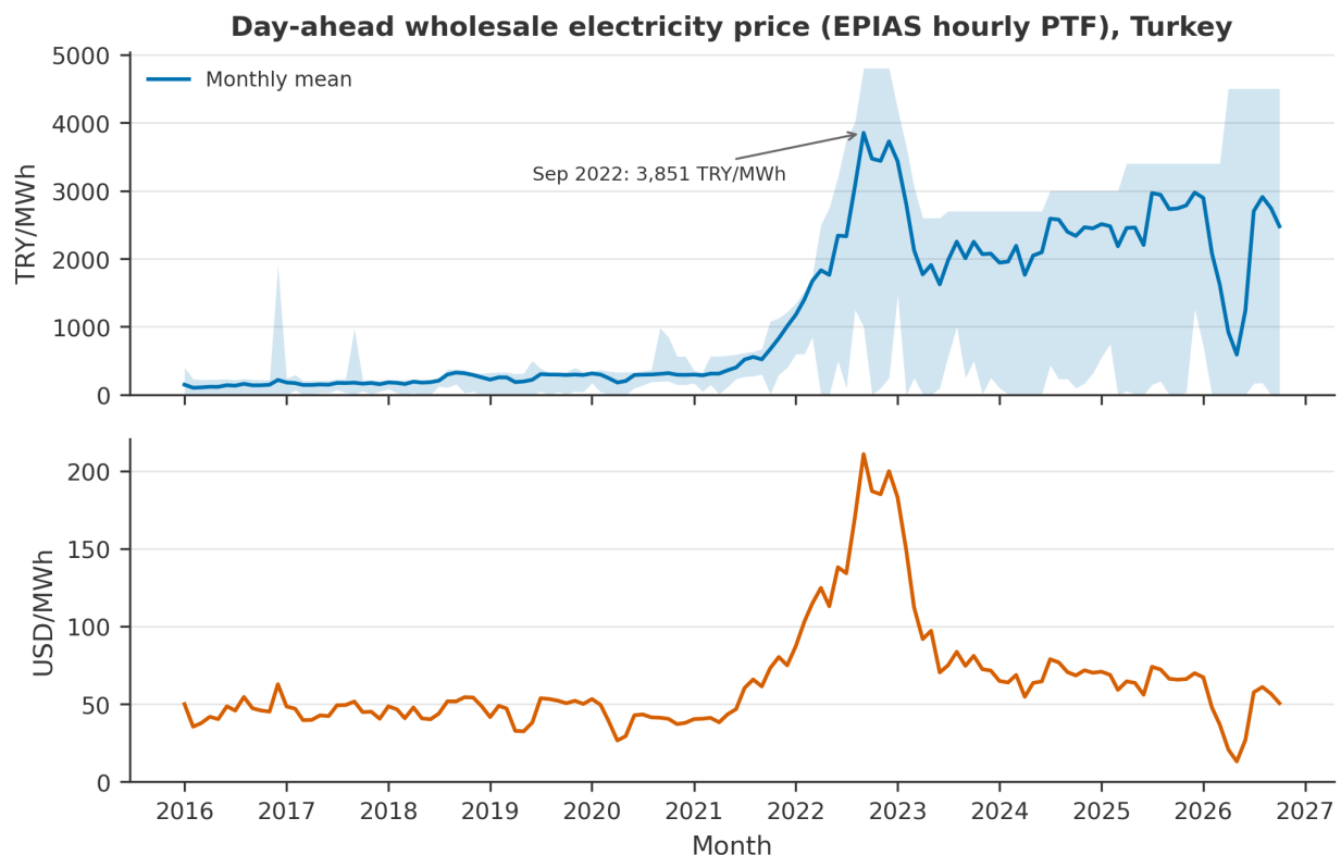
Figure 6. Day-ahead wholesale price from EPIAS hourly PTF: monthly mean (line) with monthly min-max band, in TRY/MWh (top) and USD/MWh at the Central Bank indicative rate (bottom), January 2016–October 2026
