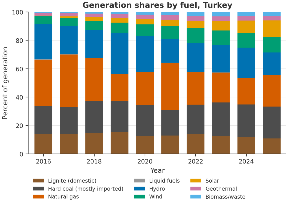
Figure 2. Generation shares by fuel, Turkey, 2016–2025 (percent)
