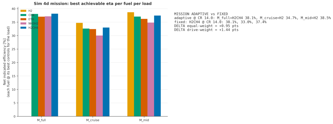
Figure 3: Load-matched mission comparison: adaptive fuel/ \lambda scheduling versus the best single fixed fuel. The cruise and mid-load gains come from hydrogen's exclusive access to the ultra-lean regime.
