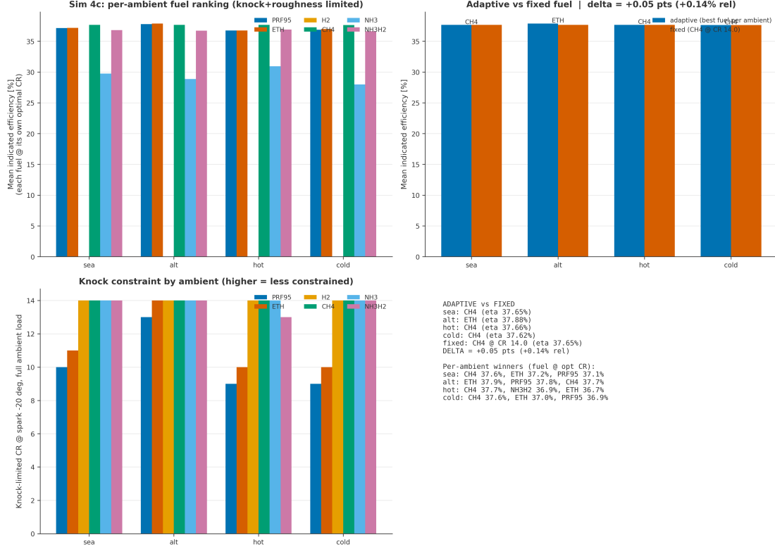
Figure 2: Efficiency ranking by fuel and ambient, each at its own knock/roughness-limited optimum. The winner switches with ambient, but adaptive selection gains only +0.05 points over the best fixed fuel.
