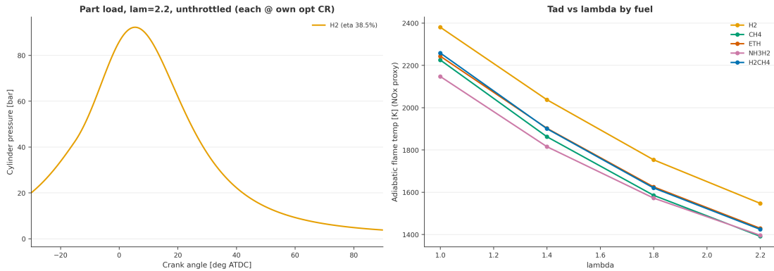
Figure 4: Lean operation at \lambda = 2.2 , unthrottled: only the hydrogen trace (left) completes combustion in the available window, and adiabatic flame temperature falls with \lambda for every fuel (right). At \lambda \approx 2 only hydrogen-containing fuels remain feasible: regime access, not burn shaping, is the prize.
