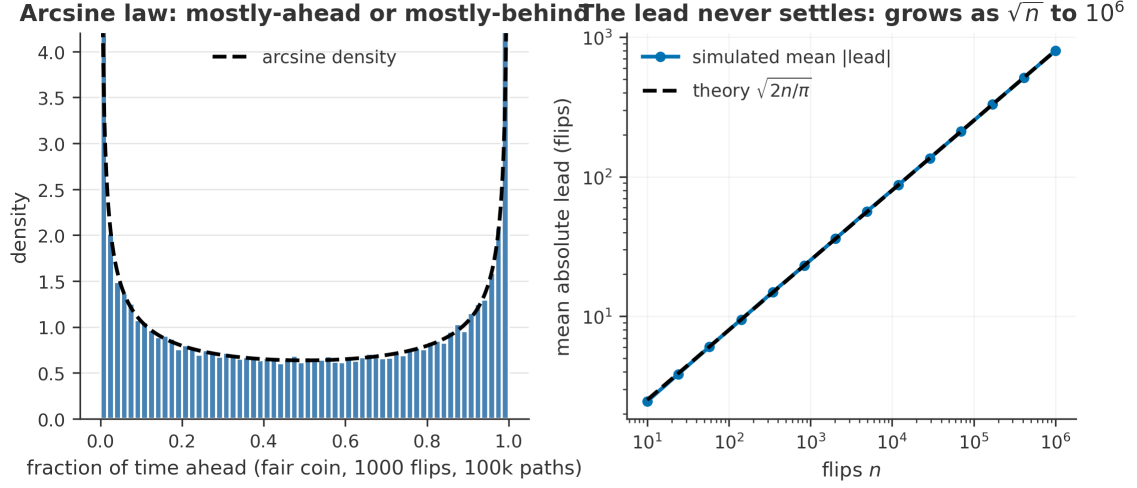
Figure 2: Zero-edge coin. Left: arcsine law for the fraction of time ahead (1000 flips, 100k paths). Right: mean absolute lead grows as \sqrt{n} without bound, verified to 10^6 flips.
