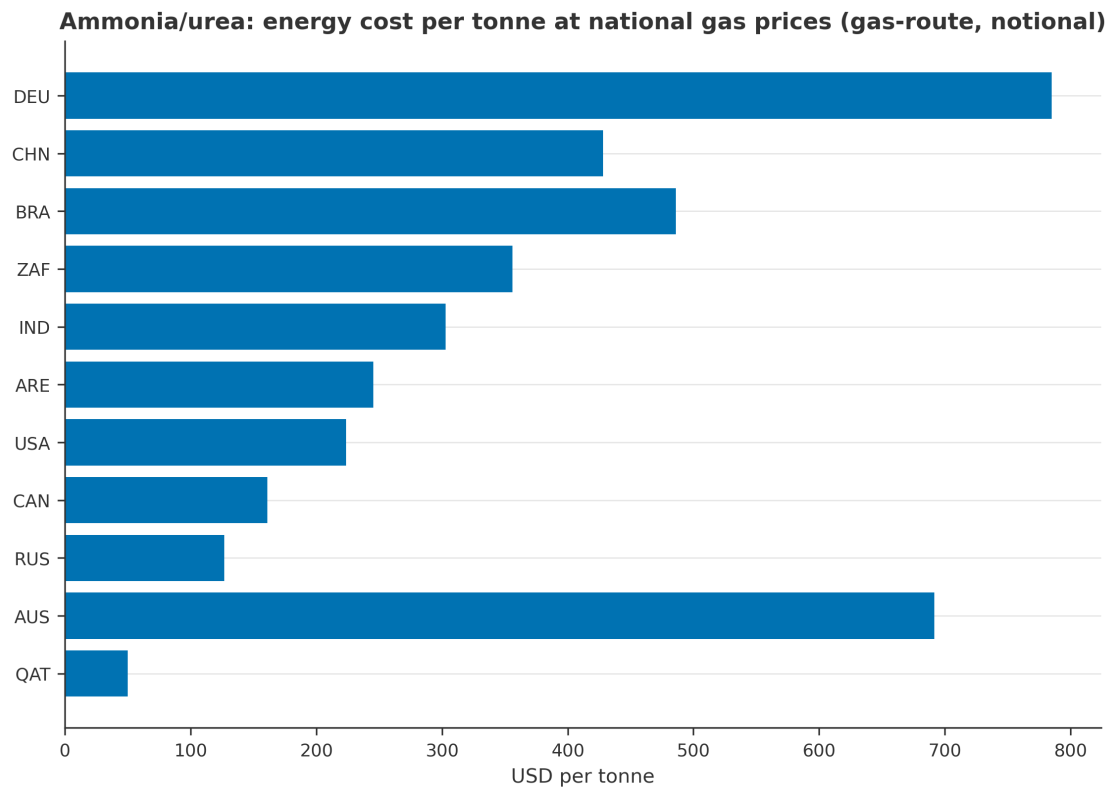
Figure 8. Ammonia and urea: energy cost per tonne at national industrial gas prices. Gas-route only; coal-based production (notably China) is not represented. Rows are notional where gas is a thermal proxy.
