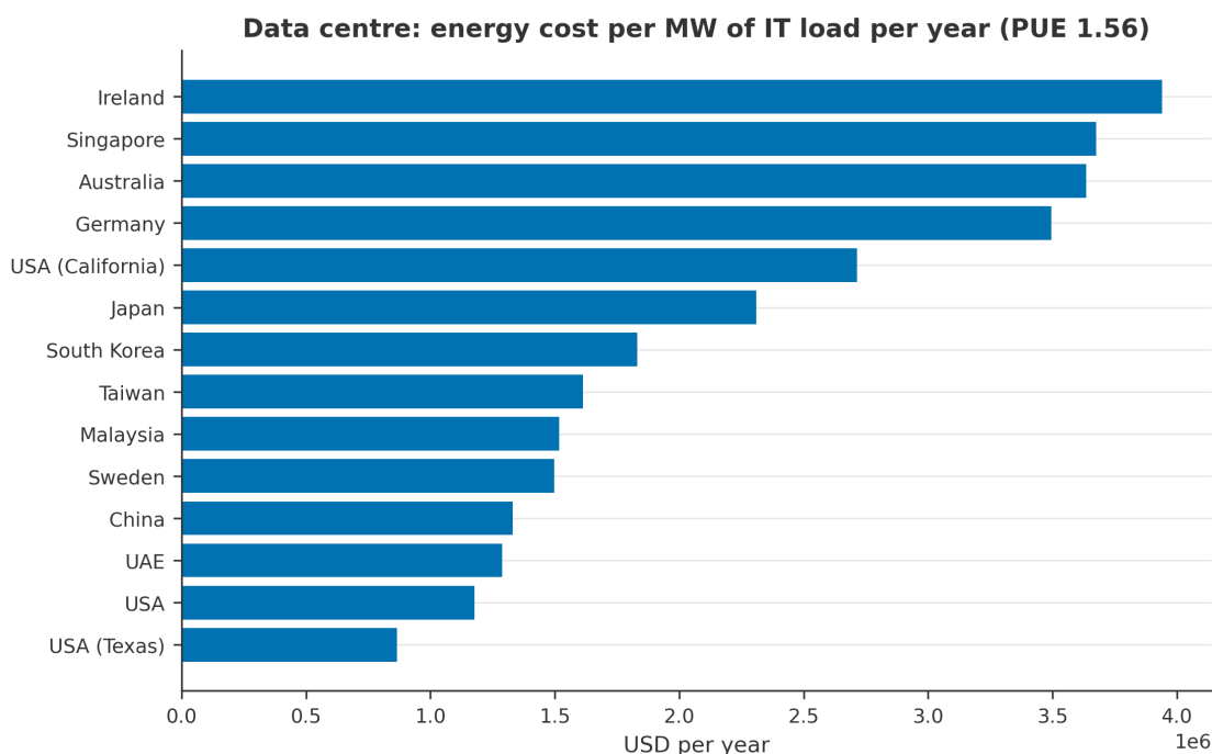
Figure 9. Data centres: annual grid electricity cost per MW of IT load at fleet-average PUE 1.56. Efficiency (PUE) varies little across countries; the tariff is the business case.
