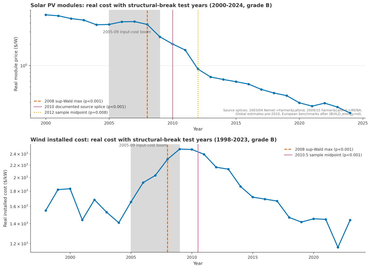
Figure 5: Break timelines for solar PV modules (2000–2024) and wind installed cost (1998–2023), log scale. Solar: 2008 sup-Wald argmax, 2010 documented source splice, 2012 midpoint (2004 skipped: too few obs.). Wind: 2008 sup-Wald argmax, 2010.5 midpoint (1998 skipped: Q-sample starts 1998). Grey band 2005–09: commodity input-cost boom (LBNL notes). Sup-Wald p -values Andrews-(1993)-approximate.
