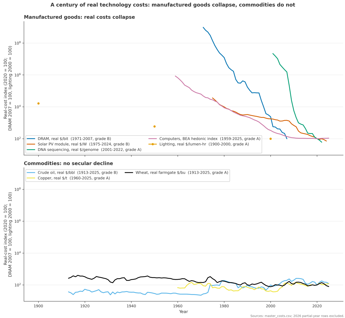
Figure 1: Long-run real-cost indices (2020 = 100, log scale) for eight representative series (upper panel: manufactured goods; lower panel: commodities). DRAM ($/bit, 1971–2007) is indexed to 2007 = 100; UK lighting (£/million lumen-hours) rests on three reconstructed benchmark years (1900, 1950, 2000), shown as markers. Solar PV pre-2010 values are global estimates vs. European market benchmarks after 2010 (source splices 2003/04 and 2009/10); OWID crude carries benchmark splices from 1987. All 2026 partial-year rows excluded. See captions and build reports for full provenance.
