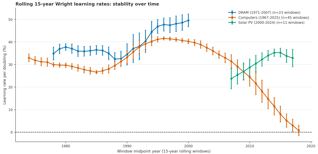
Figure 3: Rolling 15-year Wright learning rates ( LR = 1 - 2^b ; \pm 1.96 \cdot SE delta-method bands, approximate) for DRAM (23 windows), computers (45), and solar PV (11). DRAM's rate is stable and rises in late windows; computers' rate fades toward zero as the hedonic index flattens; solar's is stable around 0.24–0.35. Short windows: for stability inspection only.
