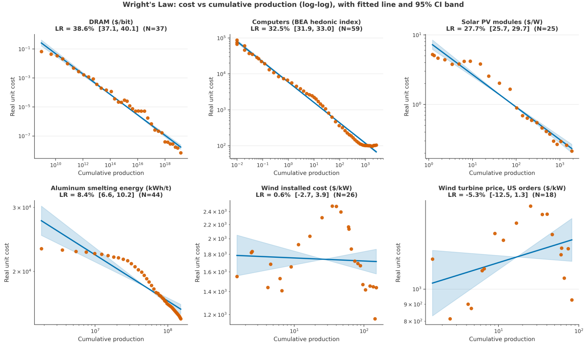
Figure 2: Wright's Law: log real unit cost vs. log cumulative production for the six Wright-eligible technologies, on the exact estimation samples. OLS fits with 95% CI bands (HC1 slope CI through the sample centroid); panel titles annotate LR = 1 - 2^b . Computers 1959–66 rows ( Q = 0.00 , cumsum rounding artifact) excluded; wind turbine panel is US orders only (1998–2016). Q proxies are deployment/investment series (see text); the computers “cost” is a hedonic index; LBNL turbine medians are noisy annual order samples.
