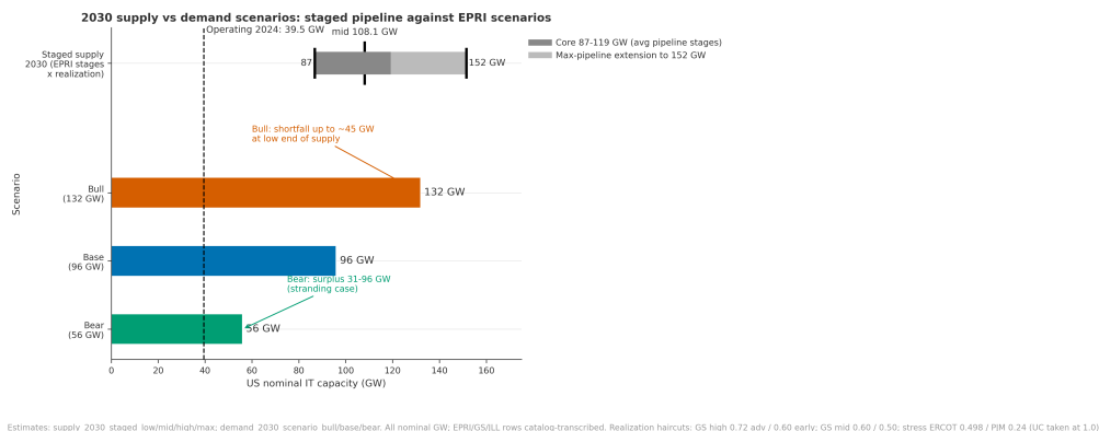
Figure 5: 2030 US nominal IT capacity: staged supply vs. EPRI demand scenarios (GW). Demand bars: bear 56, base 96, bull 132 GW (demand_2030_scenario_bear/base/bull, epri_us_nominal_it_capacity_scenario_low/medium/high 2030-01-01, grade A catalog-transcribed). Supply bar: staged 2030 range 87–152 GW, core 87–119 GW (hatched; avg-pipeline stages × realization factors), mid path 108.1 GW tick, light-gray extension to 152 GW (max-pipeline variants); estimates supply_2030_staged_low/mid/high/max (86.9/108.1/119.3/151.5 GW). Dashed line: operating 39.5 GW in 2024 (epri_us_nominal_it_capacity_operating, grade A catalog-transcribed). Realization haircuts as published: GS high 0.72 advanced / 0.60 early, GS mid 0.60 / 0.50, stress ERCOT 0.498 / PJM 0.24; under-construction taken at 1.0. Readings: bull leaves a shortfall up to ~45 GW at the low end of supply; base roughly balanced (~12 GW headroom at mid); bear implies 31–96 GW structural surplus (the stranding case). Caveats: all EPRI/GS/JLL capacity rows are catalog-transcribed (“transcribed from catalog, verify from primary”); all values nominal GW.
