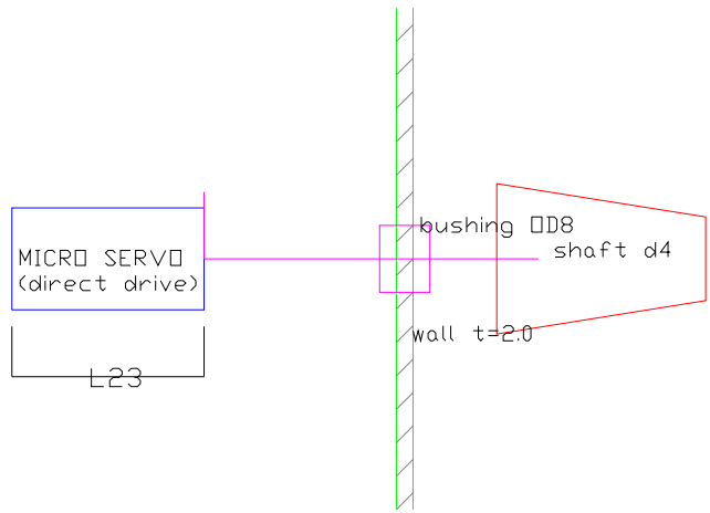
VIEW 2 - SERVO/CANARD ASSEMBLY (sectioned) Scale 1:1 (units: mm)
