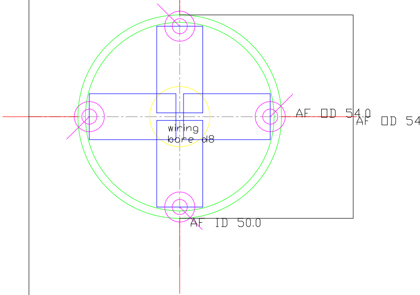
VIEW 3 - BULKHEAD / SERVO SLED PLATE (qty 2, front & rear) Material: 4mm plywood or G10, Scale 1:1 (mm)
