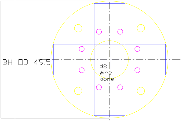
VIEW 3 - BULKHEAD / SERVO SLED PLATE (qty 2, front & rear) Material: 4mm plywood or G10, Scale 1:1 (mm)
