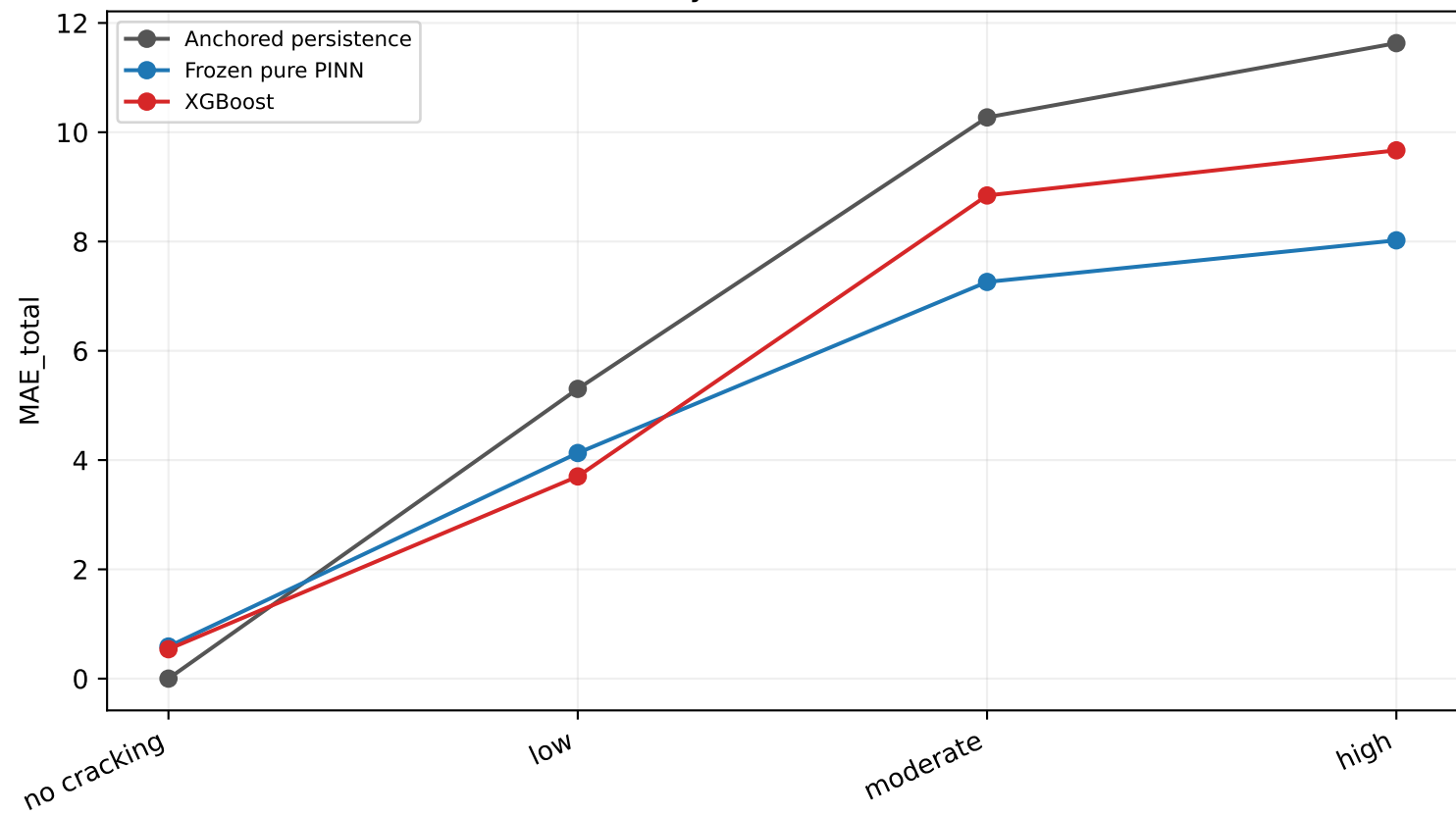
Error by anchor condition
