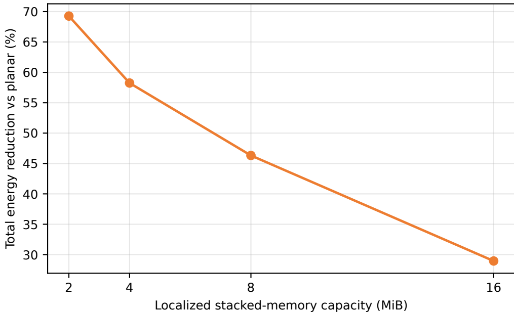
3D-proxy capacity sensitivity (AlexNet CONV1)
